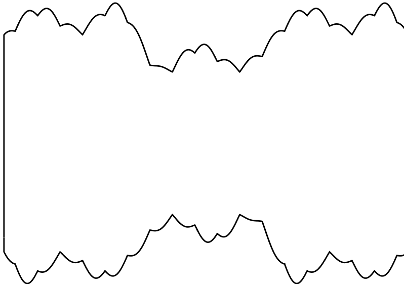
Figure 6: The domain \Omega_4 , formed from the graph of two Lipschitz functions.
