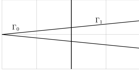
Figure 1: The rank of interaction of the two curve segments \Gamma_0 and \Gamma_1 under the potential theoretic kernels considered in this paper is low regardless of the angle of the corner.
