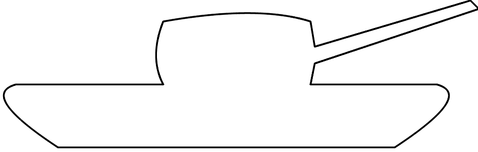
(c) The “tank” domain \Omega_3 .
