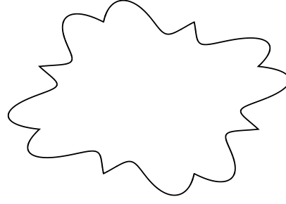
(b) The “inkblot” domain \Omega_2 .
