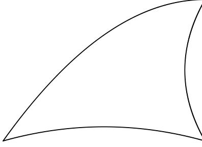
Figure 4: The “shark’s fin” domain \Omega under consideration in Section 7.1.2.
