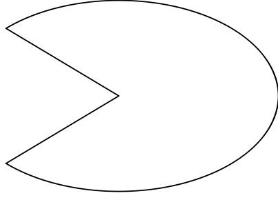
(a) The “Pacman” domain \Omega_1 .
