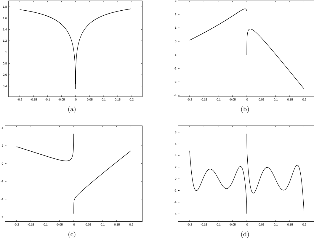
Figure 3: Four charge basis functions used in the discretization of a Laplace Neumann boundary integral equation on the contour \partial\Omega_3 .
