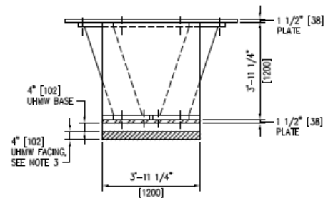
TOP VIEW OF FENDER SYSTEM (A4) SCALE: 1/2" = 1'-0"
