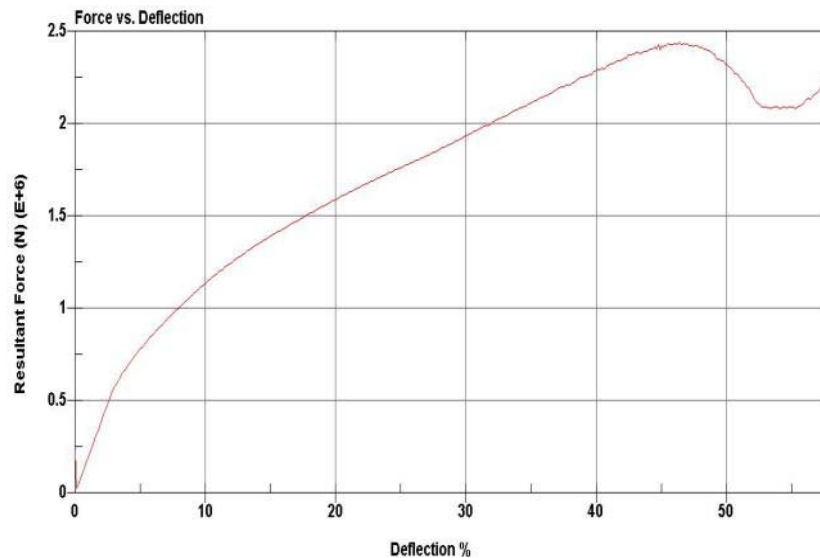
Figure 4-6. FEM Performance of Biaxial UE Fender
