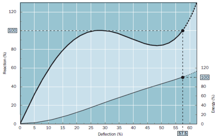
Figure 4-2. Rated Performance of Trelleborg Fender Elements
