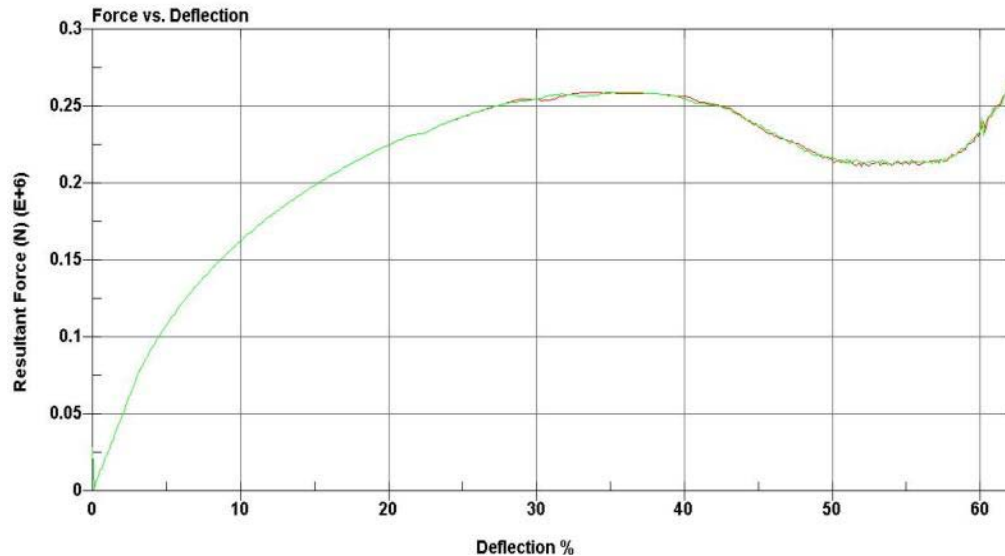
Figure 4-4. FEM Performance of MV1000x900B Elements
