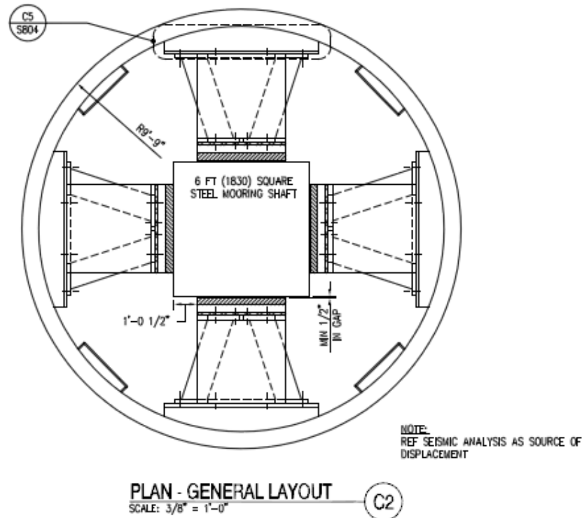
Figure 1-5. FDDP Fender – General Layout
