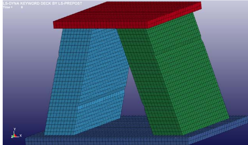
Figure 2-1. Uniaxial Fender Composed of MV1000x900B Elements
