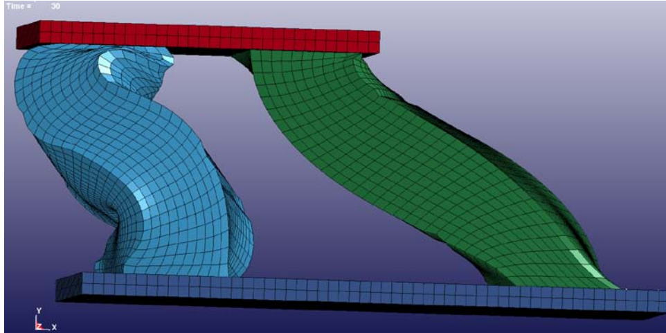
Figure 5-2. FEM Uniaxial Fender Sideway Collapse
