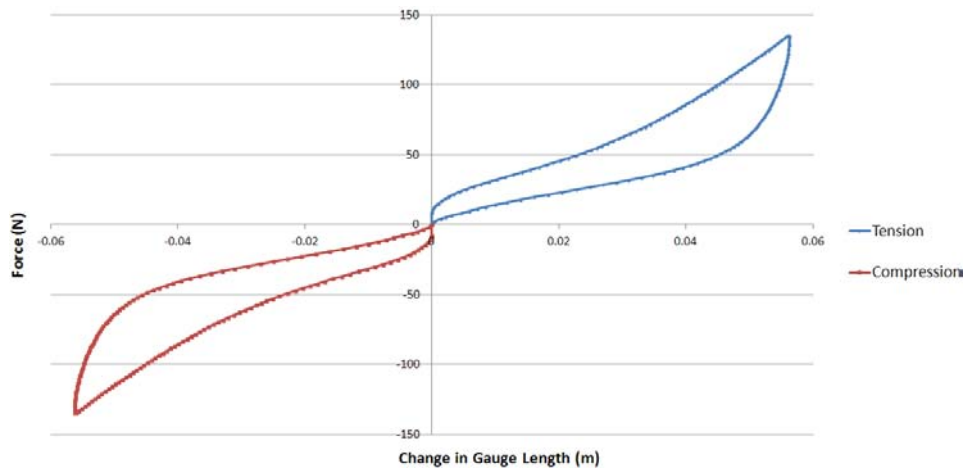
Figure 3-2. Loading/Unloading Curve for A60 Compound
