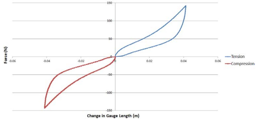
Figure 3-4. Loading/Unloading Curve for A70 Compound
