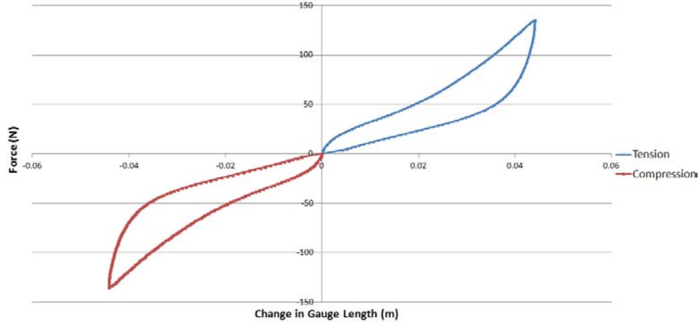
Figure 3-3. Loading/Unloading Curve for A65 Compound
