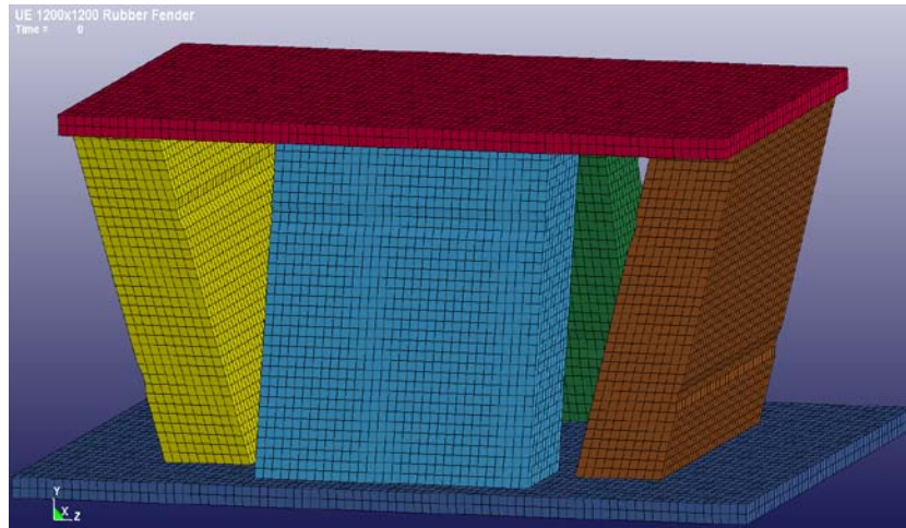
Figure 2-2. Biaxial Fender – Composed of UE1200x1200E3.1 Elements
