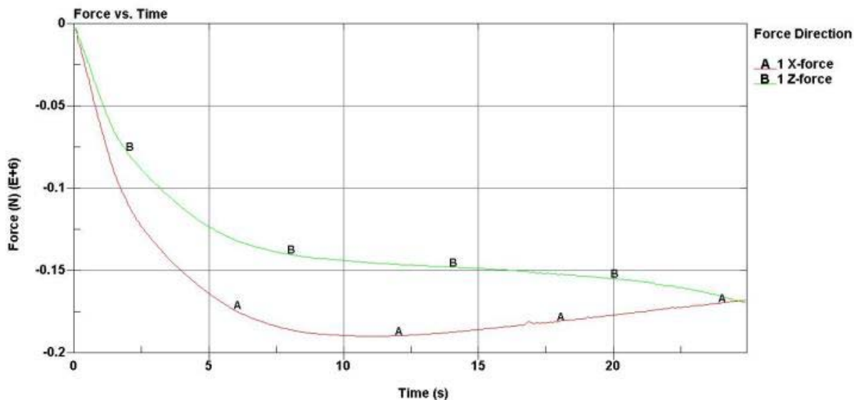
Figure 5-5. Biaxial Fender Reaction Forces in x- and z-directions
