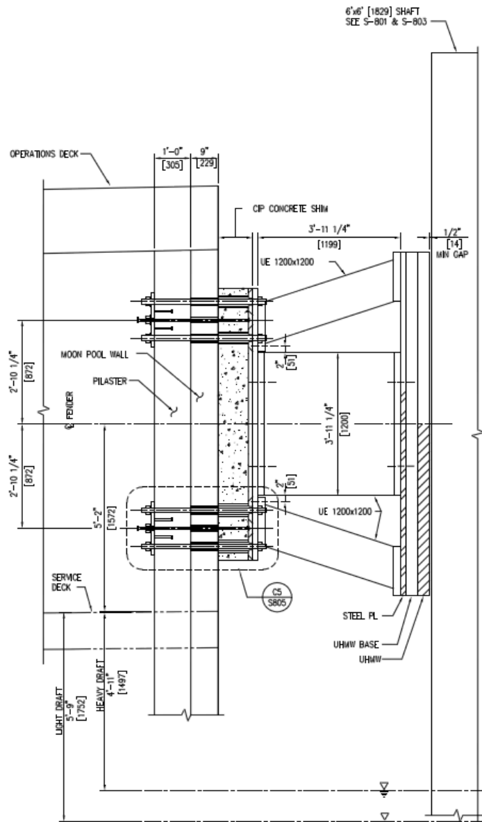
ELEVATION VIEW OF FENDER SYSTEM (A2) SCALE: 3/4" = 1'-0"
