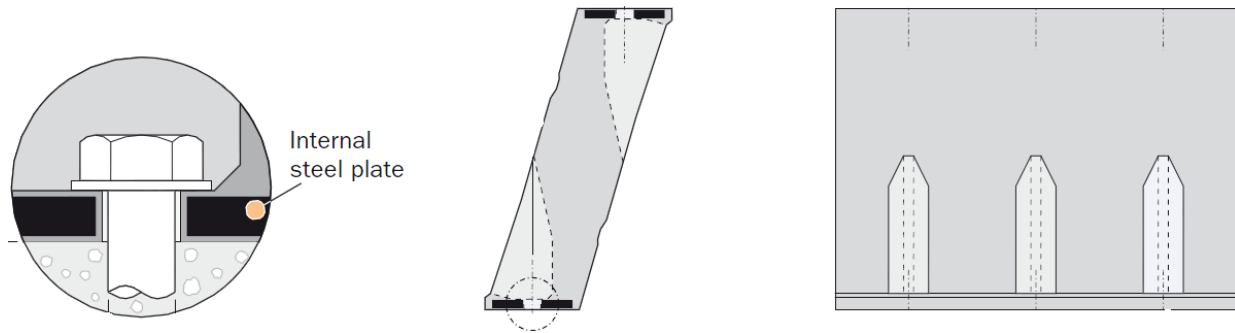
Figure 2-3. Illustration of Steel Plate Inside Fender Element
