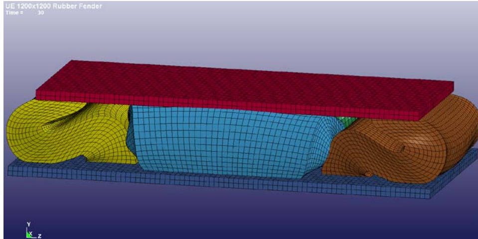
Figure 4-5. Biaxial UE1200x1200E3.1 Fender Deflection
