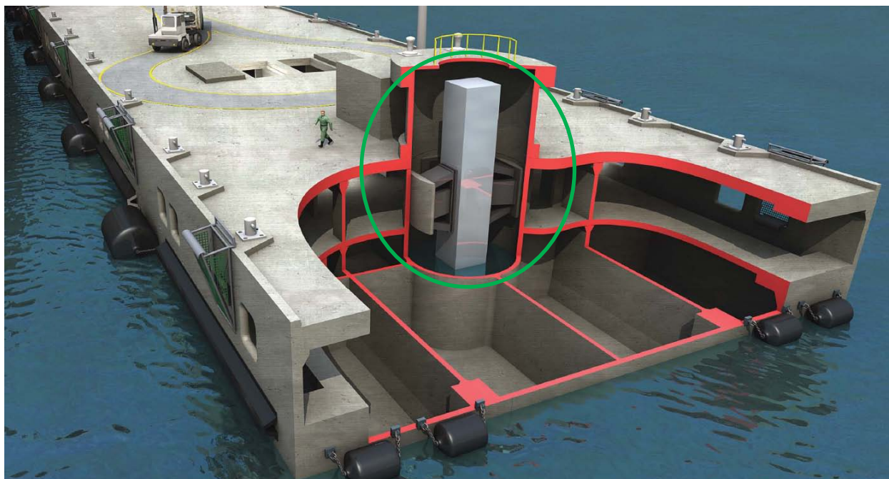
Figure 1-1. FDDP Fenders and Mooring Shaft
