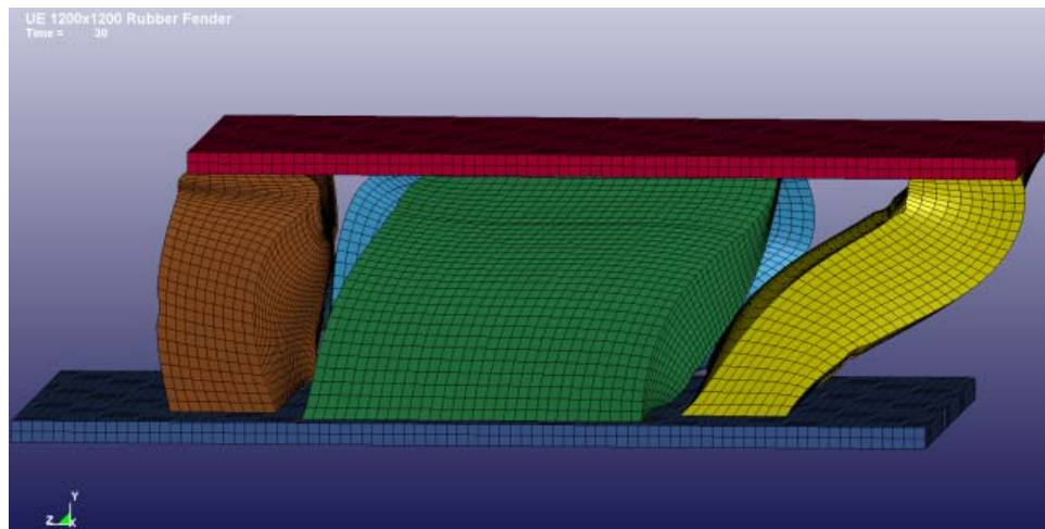
Figure 5-4. FEM Biaxial Fender Sideway Collapse
