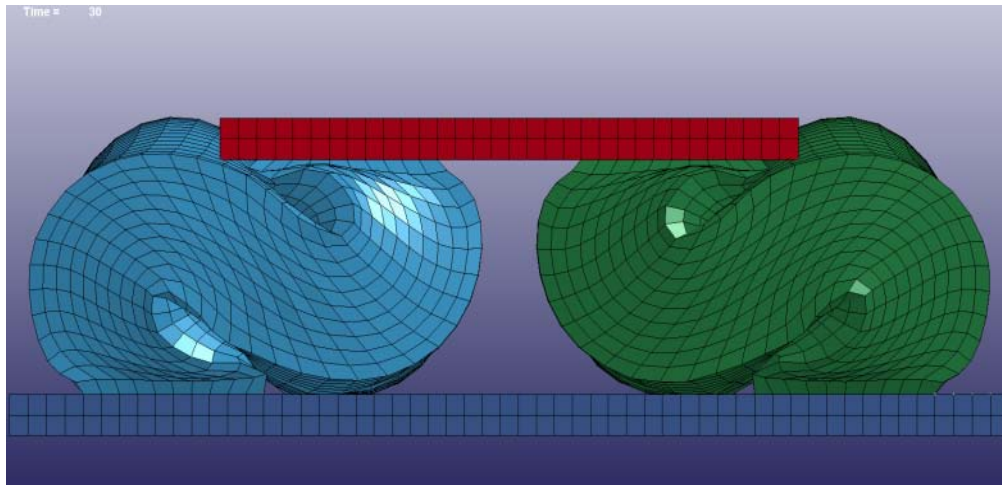
Figure 4-3. Uniaxial MV1000x900B Fender Deflection
