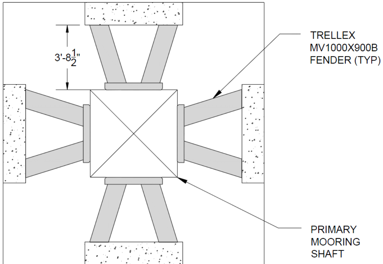
Figure 1-2. Plan View of MHP Fender System
