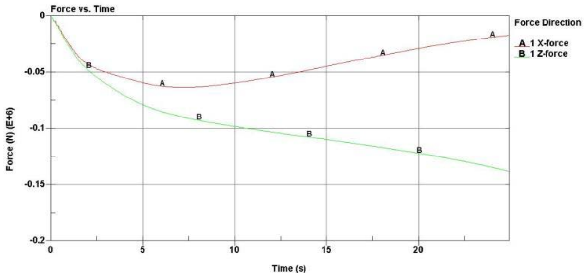
Figure 5-3. Uniaxial Fender Reaction Forces in x- and z-directions
