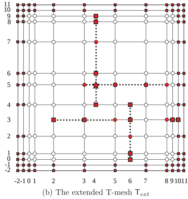
Figure 4: A T-mesh and the corresponding extended T-mesh. The face extension edges which have been added to \mathcal{T} are denoted by the dotted black lines. The crossing vertices are denoted by red stars, the overlap vertices are denoted by red hexagons, and the extended vertices are denoted by red squares. Notice that the inactive vertices are also extended vertices. The active vertices are denoted by hollow circles and the T-junctions are denoted by red circles.
