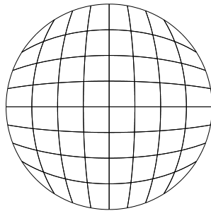
(b) n_{el} = 4
