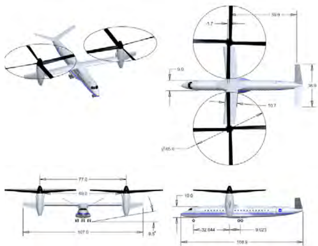
Figure 1. NASA Large Civil Tilt-Rotor (LCTR2)
