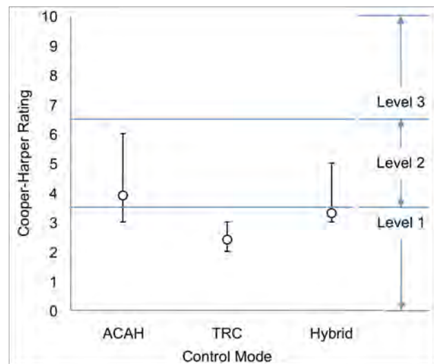
Figure 17. Comparison of the handling qualities ratings for the ACAH, TRC and Hybrid response type control configurations in the Lateral Reposition.
