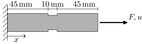
Figure 3: Schematic representation of a one-dimensional rod loaded in tension. The cross-sectional area of the rod is 10 \text{ mm}^2 except for the central section where it is equal to 9 \text{ mm}^2 .
