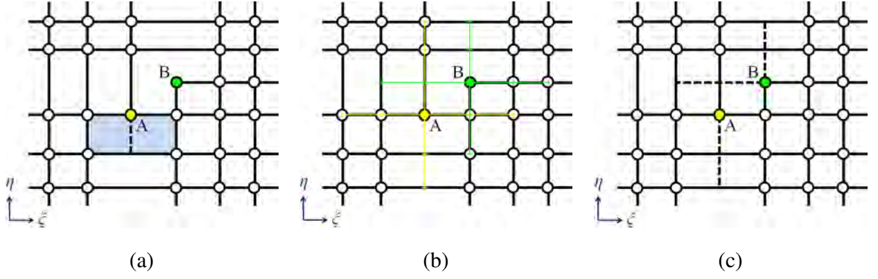
Fig. 13. Inferring the Bézier mesh from a T-mesh in 2D. (a) A local region of a T-mesh with one T-junction A and one L-junction B; (b) the T-mesh with all the knot vector inference lines for nodes A and B; and (c) the Bézier mesh.
