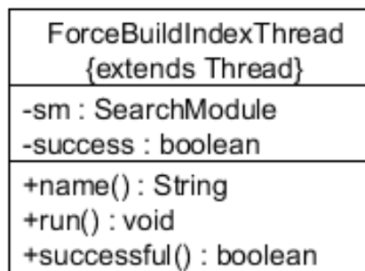
Figure 21. UML ForceBuildIndexThread Class Model
