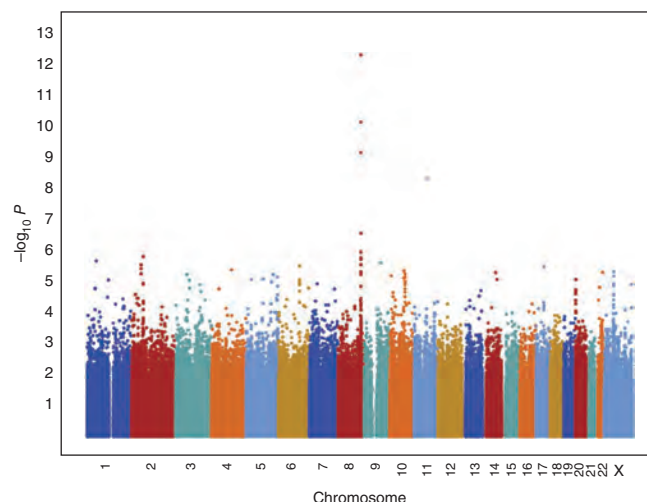
Figure 1 A plot of the -\log_{10} P values by chromosome.
