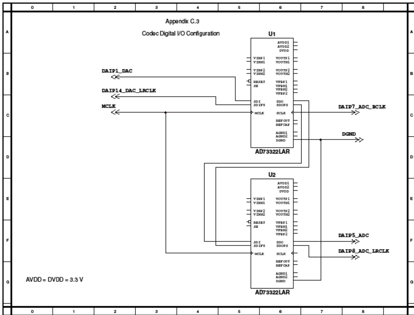
Figure C.3 The digital I/O section connects the codecs to the processor.
