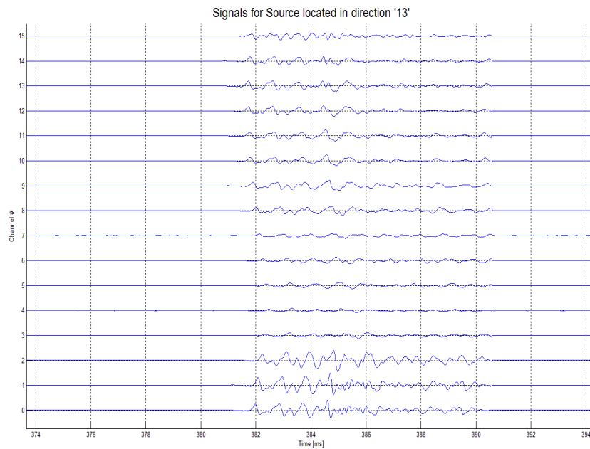
Figure D.10 Recorded data for a source close to channel 13. Channels 0 through 2 are configured with a higher gain.
