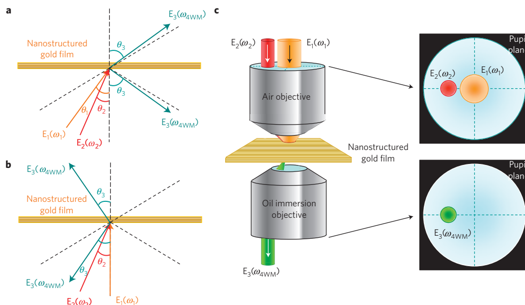
Figure 1 | Schematics of the degenerate 4WM process on a thin nonlinear film. a , The general case with arbitrary incidence angles of the pump ( \omega_1 ) and probe ( \omega_2 ) beams. The directions of the forward and backward 4WM waves are determined by the in-plane phase matching condition. b , The special case with normal incidence ( \theta_1 = 0 ) of the pump beam. The forward nonlinear 4WM beam exhibits negative refraction relative to the probe beam. The ratio between the sines of the incident probe beam angle and the refracted angle of the 4WM wave is a constant that depends only on the ratio of the two wavelengths. c , Schematic illustration of the experimental set-up. Two objectives with large back apertures are confocally aligned and serve as Fourier transform lenses converting the spatial positions of the beams, relative to the back aperture of the lenses, to the propagation directions of the wavevectors in k -space, and therefore to the incidence or refracted angles. Both the pump and probe beams are launched through the top air objective at different incidence angles, which can be precisely determined by mapping the partial reflection from the lens. The oil immersion objective collects the nonlinear generated photons at the 4WM frequency in the forward direction. Imaging the pupil plane of the objectives provides a measurement of both the refracted and incidence angles with an accuracy limited only by the ratio between the physical size of the actual beam and the diameters of the back aperture of the objective. Furthermore, the beam with the smallest physical size determines the area of nonlinear interaction, and hence impacts the image quality because of the increased divergence in wavevector for a small sized illumination beam.
