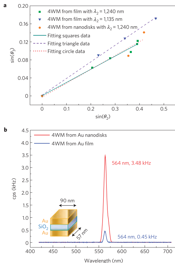
Figure 3 | Four-wave mixing analysis. a , Nonlinear Snell's law of 4WM for thin gold film nanosystems at \lambda_2 = 1,240 nm (rectangles) and \lambda_2 = 1,135 nm (triangles) and a nanodisk array at \lambda_2 = 1,240 nm (circles). The incidence angle of the probe beam, \theta_2 , and the refracted angle of the 4WM signals, \theta_3 , strictly obey Snell's law, resulting in a constant ratio between their sines that depends only on the wavelengths. Linear fitting of the measurements shows good agreement with the theoretical results. The position of the probe beam and the 4WM signal are precisely determined by a Gaussian centroid fit algorithm. b , The 4WM signal generated from both the thin gold film (blue) and thin film of nanodisks (red). The forward 4WM signal obtained for the nanodisk structures is about ten times stronger than that for the thin gold film owing to the strong field confinement at localized surface plasmon resonances. The inset shows the geometry of the Au/SiO 2 /Au nanodisks examined in the experiments. To match the resonance wavelength of the pump beam the nanodisks are designed 57 nm in width and 90 nm in length with a period of 400 nm on a glass substrate. The thicknesses of both gold and SiO 2 layers are 20 nm each.
