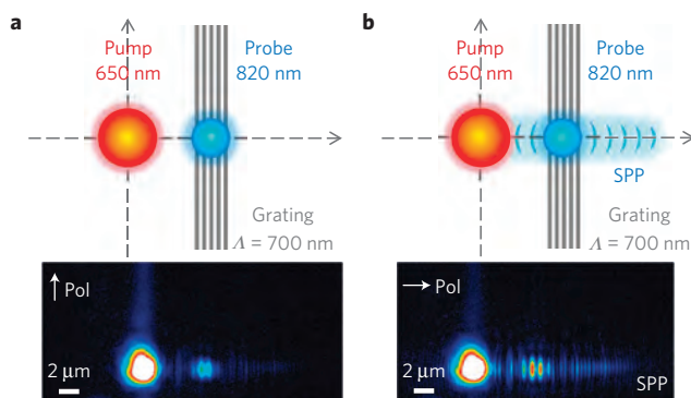
Figure 4 | Top view schematic of the experiment and the corresponding experimental images collected by a CCD positioned at the imaging plane.
