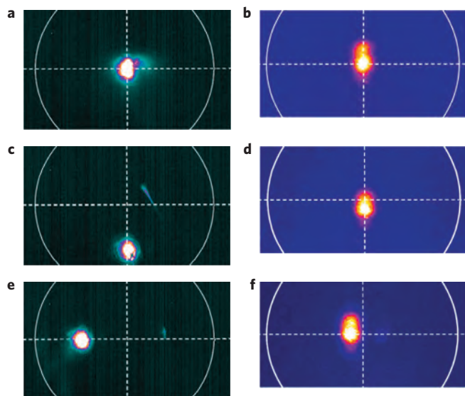
Figure 2 | Fourier plane of the detected signals. a–f , Fourier plane images of the probe beam ( a,c,e ) and the forward 4WM signal ( b,d,f ) with a probe beam wavelength of 1,240 nm. The position of the beam is directly related to the sines of the incidence or refracted angles. The incidence angles of the probe beam are \theta_2 = 0 ( a ), \theta_2 \sim 22.3^\circ ( c ), \theta_2 \sim 23.2^\circ ( e ), on a 20 nm thick gold film, while the refracted angles of the 4WM beams are \theta_3 = 0 ( b ), \theta_3 \sim 4.9^\circ ( d ), \theta_3 \sim 6.7^\circ ( f ), respectively. The positions of both the probe beam and the forward 4WM beam are located on the same side of the pupil plane images, confirming negative refraction of the generated nonlinear wave. The nonlinear refraction depicted here is polarization independent, as evident from the pupil plane images with both TE ( c,d ) and TM ( e,f ) polarized probe beams, in which the incidence angles are tuned along the vertical and horizontal directions, respectively.
