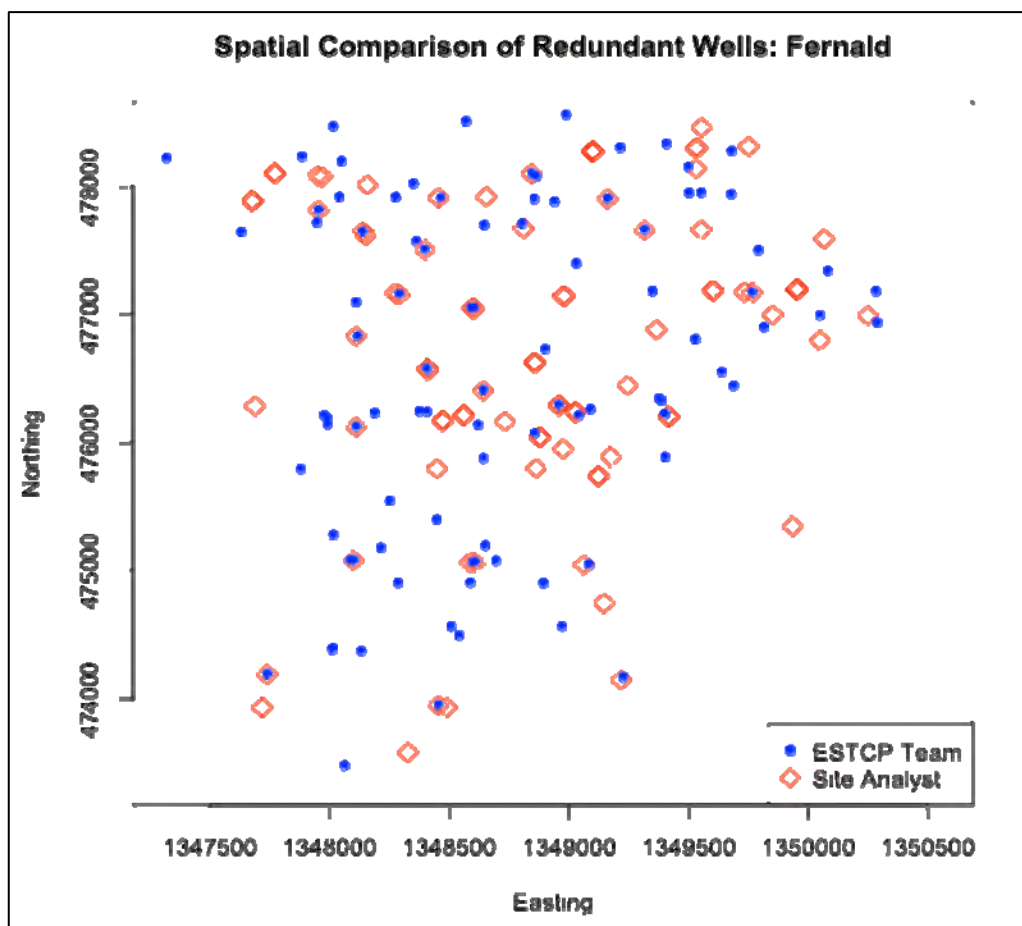
Figure 35. Spatial comparison of redundant wells — Fernald.
