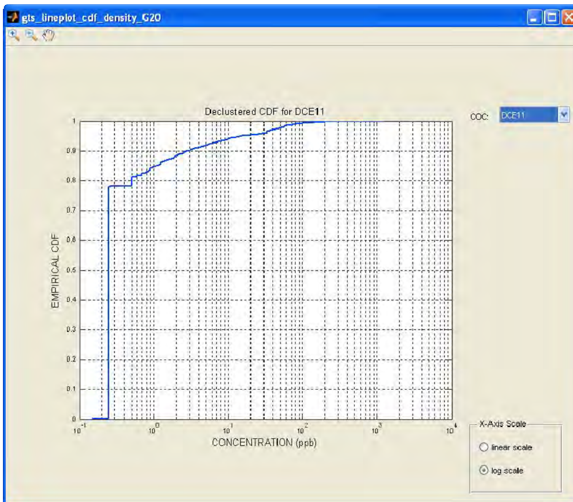
Figure 29. Example declustered cumulative distribution function in GTS.
