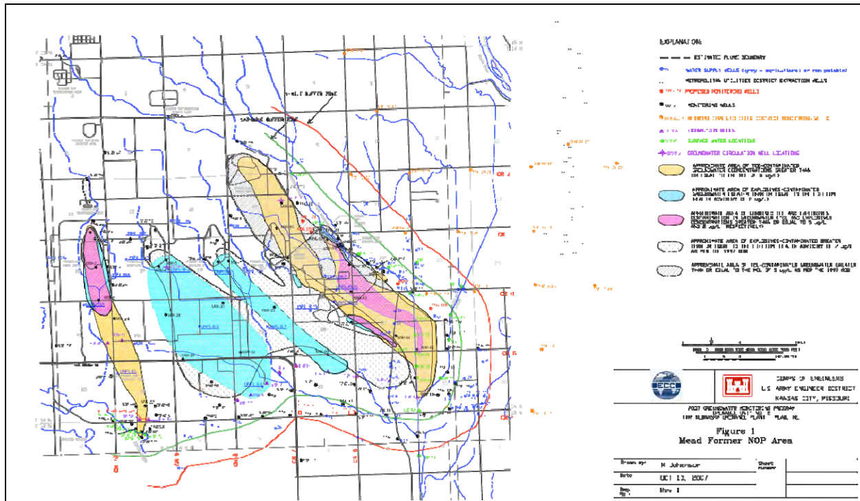
Figure 26. NOP plume extent.
