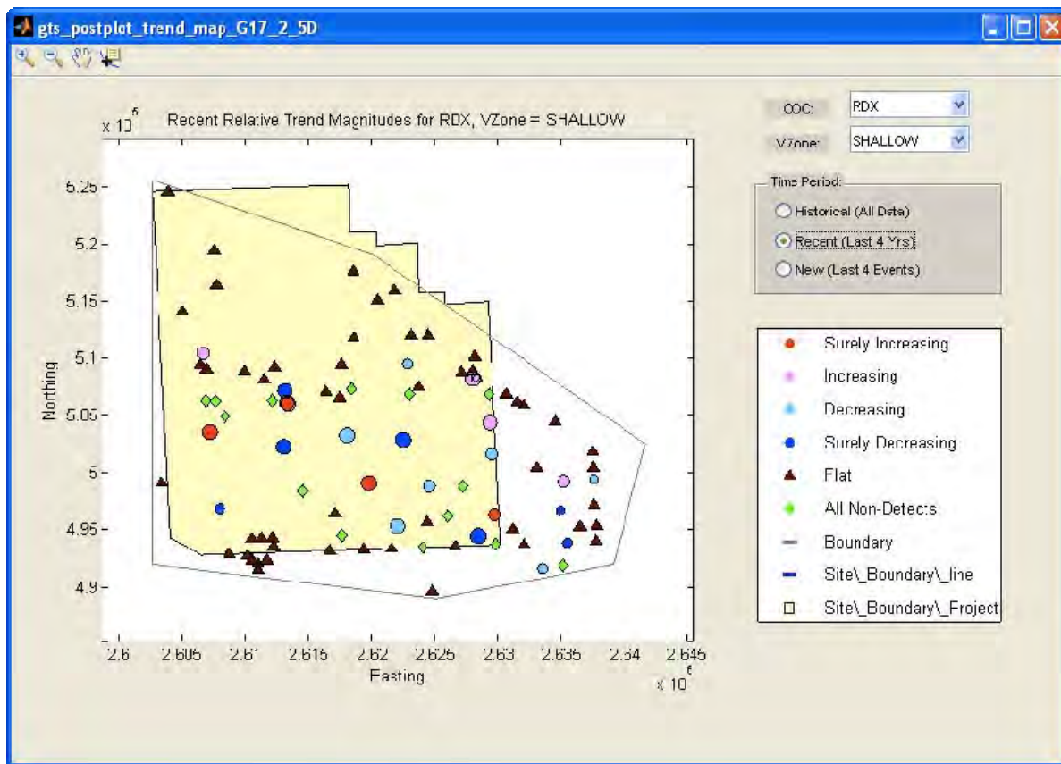
Figure 7. Example trend map in GTS.
