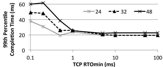
Figure 3: All-to-all Incast with varying numbers of servers connected to the same switch. RTOs less than 10 ms cause spurious retransmissions.
