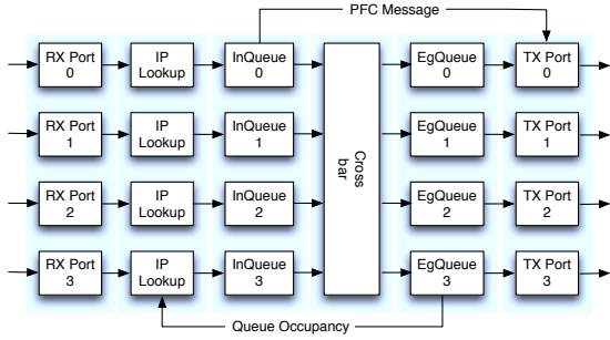
Figure 1: DeTail-compliant Switch Design
