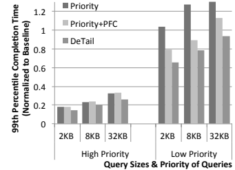
Figure 10: Simulation results with mixed query workload for varying priorities
