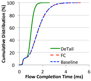
Figure 7: Distribution of completion times of 8KB queries under a steady query rate of 2000 queries/second
