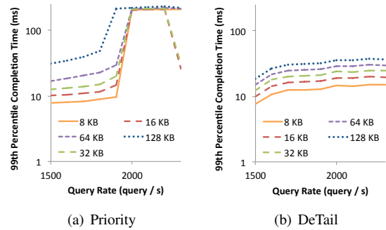
Figure 13: 99th percentile completion time in Click-based implementation
