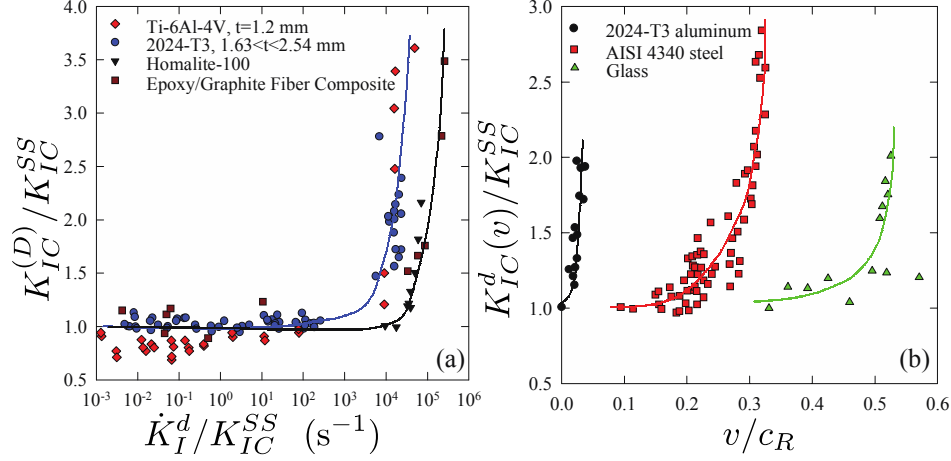
Figure 3: Normalized Dynamic Stress Intensity Factors for Several Materials
