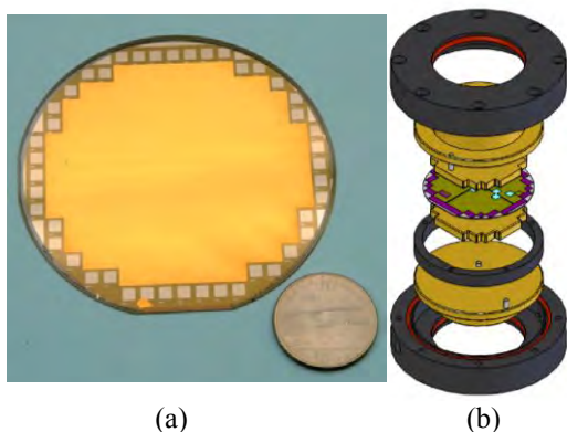
Figure 5: Photograph of the wafer-scale interconnected diode. The active area is 11.72 \text{ cm}^2 (a). Schematic of a “hockey puck” package for on-state pulsed testing (b).
