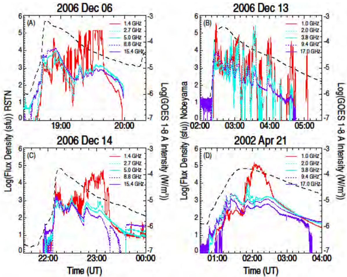
Figure 8: Great ( > 10^5 sfu) Decimetric Radio Bursts on (a) 2006 December 6; (b) 2006 December 13; (c) 2006 December 14; and (d) 2002 April 2
