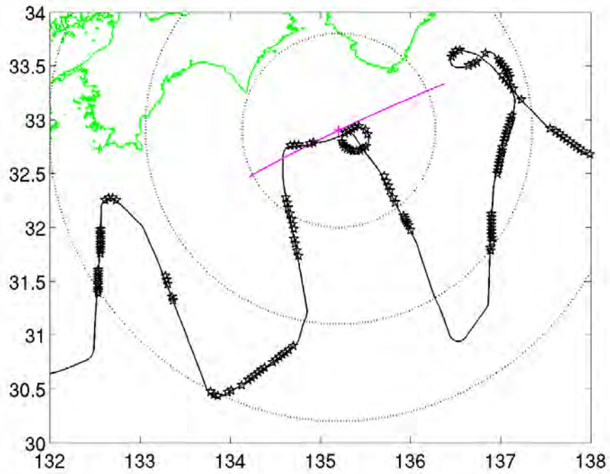
Figure 14: P-3 RF15 adjusted to 04:00 20 Sep, 2008. The stars mark the locations where DVL profiles were attempted.
