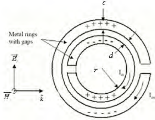
Figure 5. Coplanar ring (After [21]).
