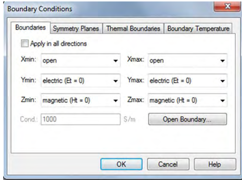
Figure 23. Boundary conditions for Model 2 Case I.
