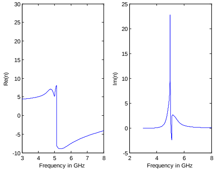
Figure 40. Extracted index of refraction of Model 2 Case III.
