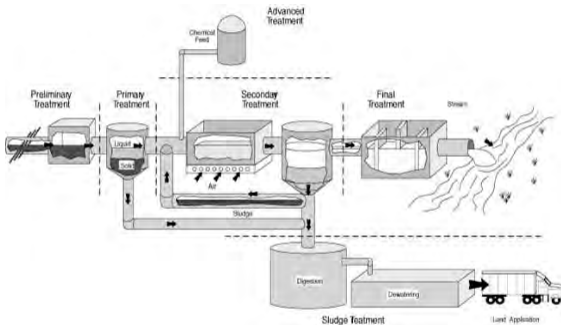
Figure 1. Wastewater Treatment Process (Mancl, 2012)
