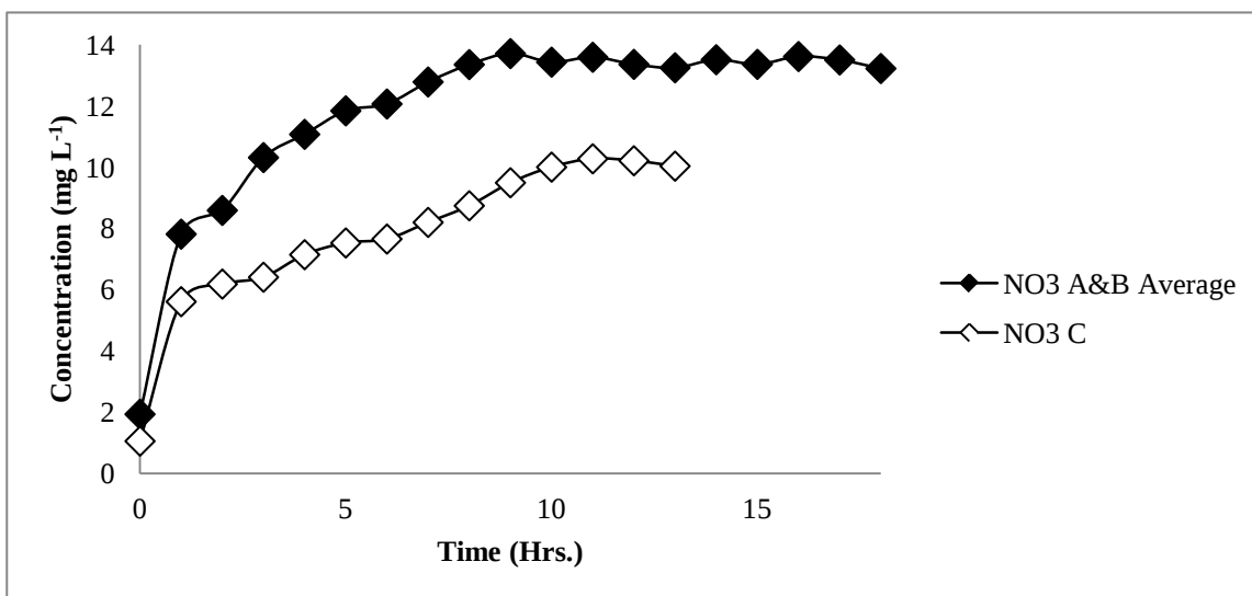
Figure 14. \text{NO}_3\text{-N} : 500 \text{mg L}^{-1} in activated sludge at 25° C with nitrifiers active
