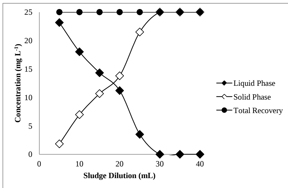
Figure 10. Sorption Kinetic Recoveries: 25 \text{ mg L}^{-1}
