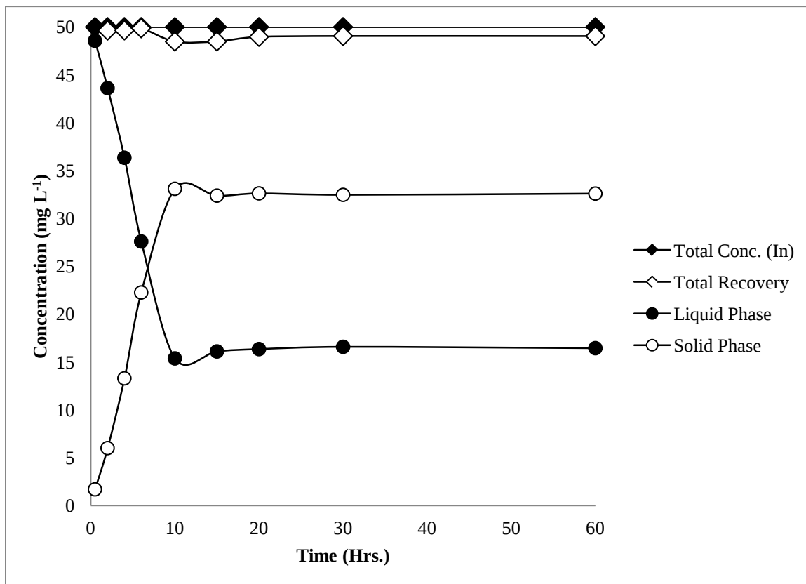
Figure 2. Propylene Glycol Sorption Kinetics: 50 \text{ mg L}^{-1} heat-inactivated AS
