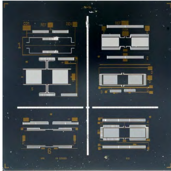
Figure 4. Photograph of generation 7 sensors with 25\mu m device layer.
