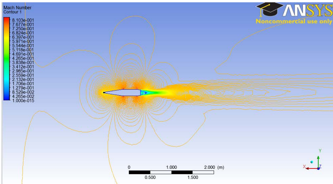
Figure 57. Mach Contour at M=0.7 , AOA of 0^\circ , IVM.
