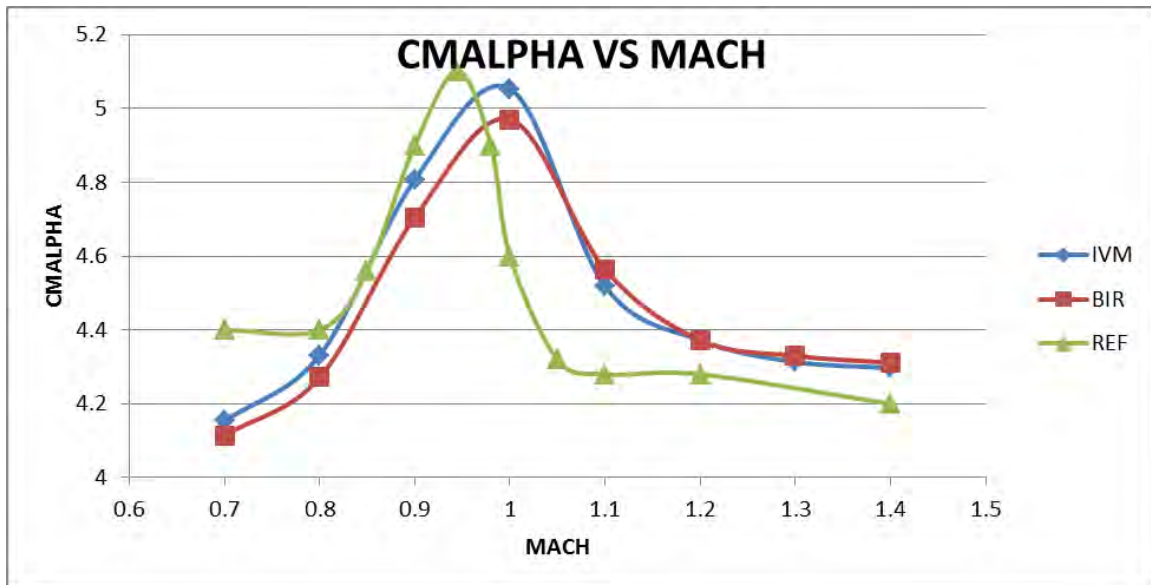
Figure 48. Comparison of Pitching Moment Coefficient Slope for IVM and BIR AOA Generation Methods.
