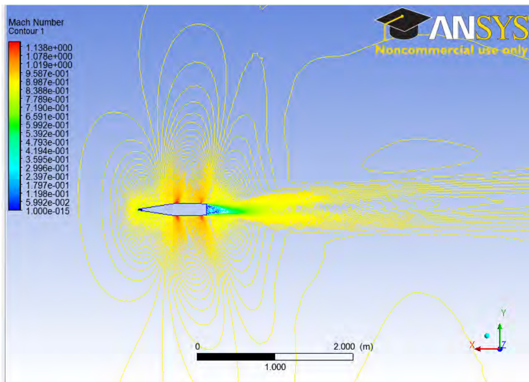
Figure 37. Mach Contour at M=0.9 , AOA of 2^\circ , IVM.
