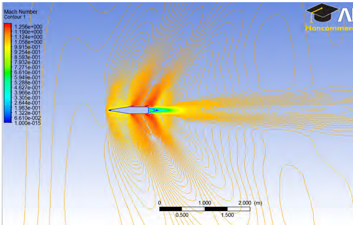
Figure 61. Mach Contour at M=1.1 , AOA of 0^\circ , IVM.
