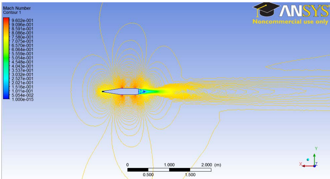
Figure 58. Mach Contour at M=0.8 , AOA of 0^\circ , IVM.
