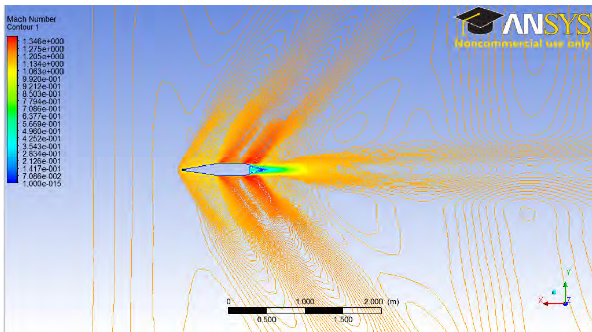
Figure 62. Mach Contour at M=1.2 , AOA of 0^\circ , IVM.
