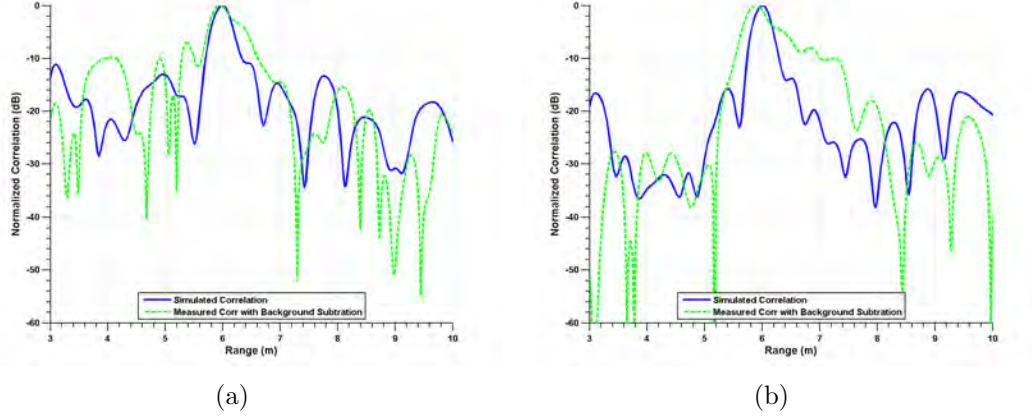
Figure 4.16. In the (a) standard AFIT RNR configuration with LPAs, the correlation results of a target at 6 meters using HH polarization are consistent. In the (b) horn-modified AFIT RNR configuration, correlation results are also consistent.
