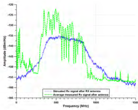
(a) Receive signal after RX antenna, TP4
