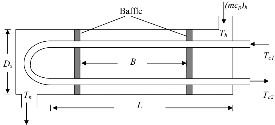
Figure 3.6: Heat Exchanger Schematic (Magrab et al., 2004)
