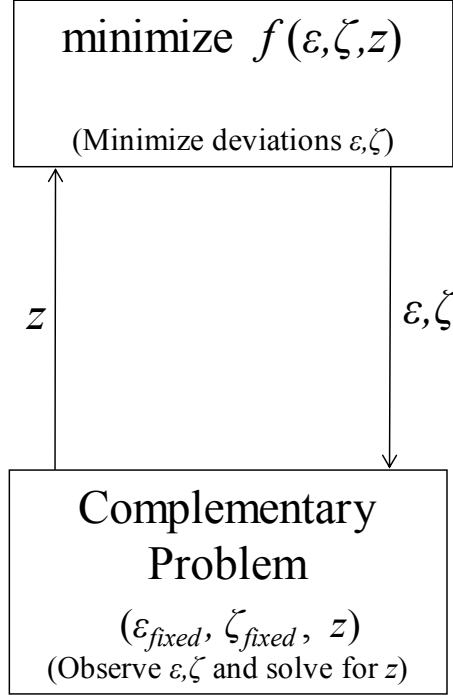
Figure 2.5: Representation of a Discretely-Constrained Mixed Linear Complementary Problem
