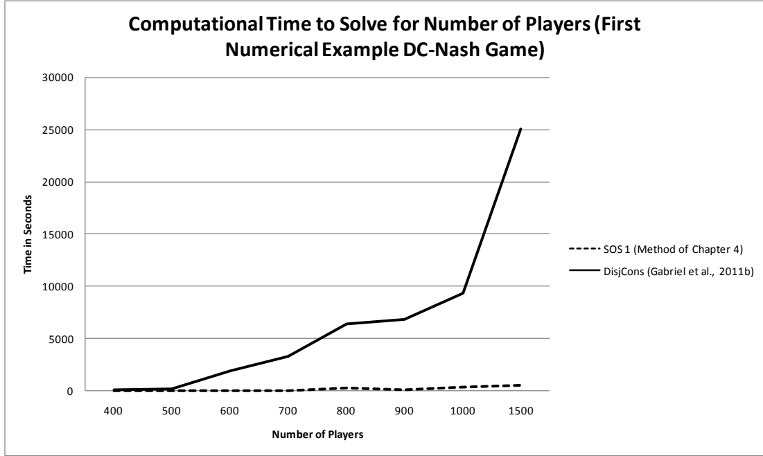
Figure 5.2: Computational Time for First Numerical Example
