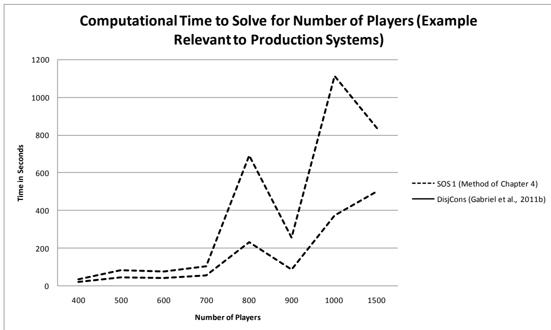
Figure 5.3: Computational Time for Example Relevant to Production Systems
