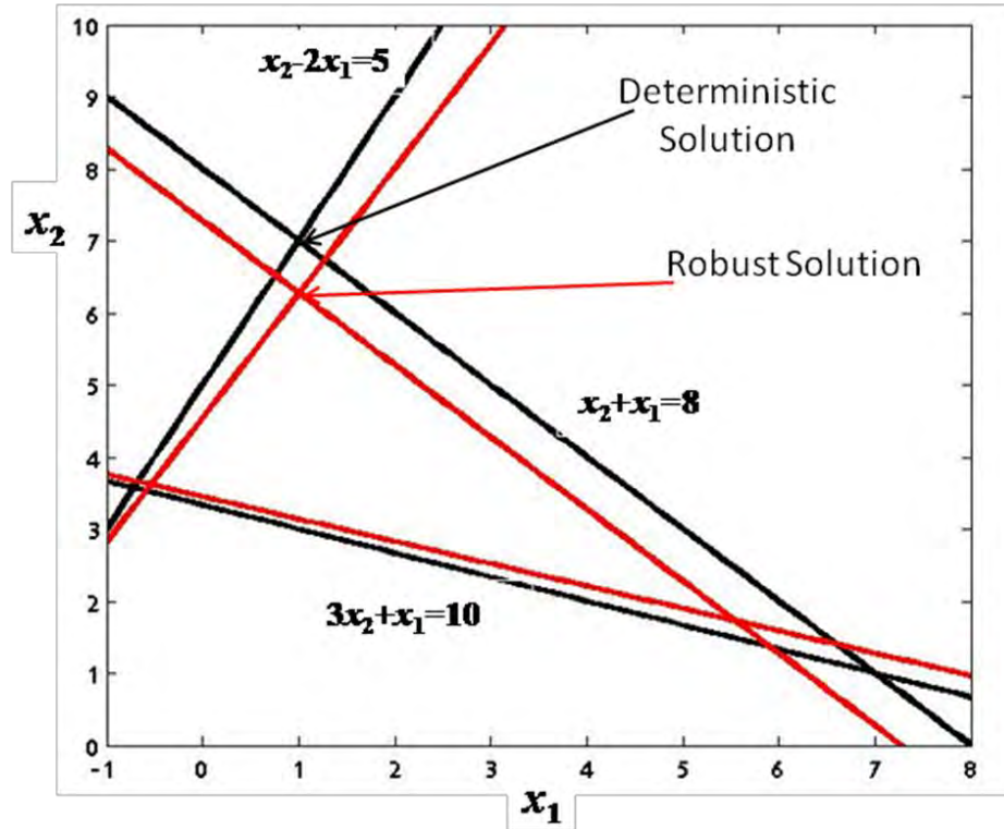
Figure 3.1: Comparison of the Feasible Region (Black) with the Robust Feasible Region (Red) 11
