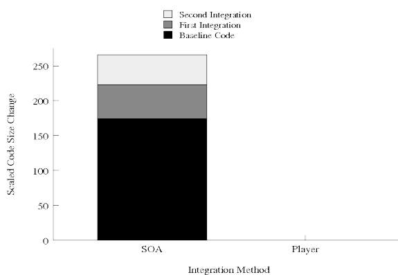
Figure 12.4: Code volume change across the baseline, first, and second integration stages for the Player module task. Detailed data for the graph was derived from the tables in Appendix I.
