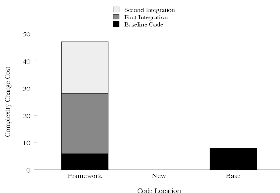
Figure 12.3: Complexity change cost by location across the baseline, first, and second integration stages for the Player module task. Detailed data for the graph can be found in Appendix I, Tables I.4, I.7, and I.11.
