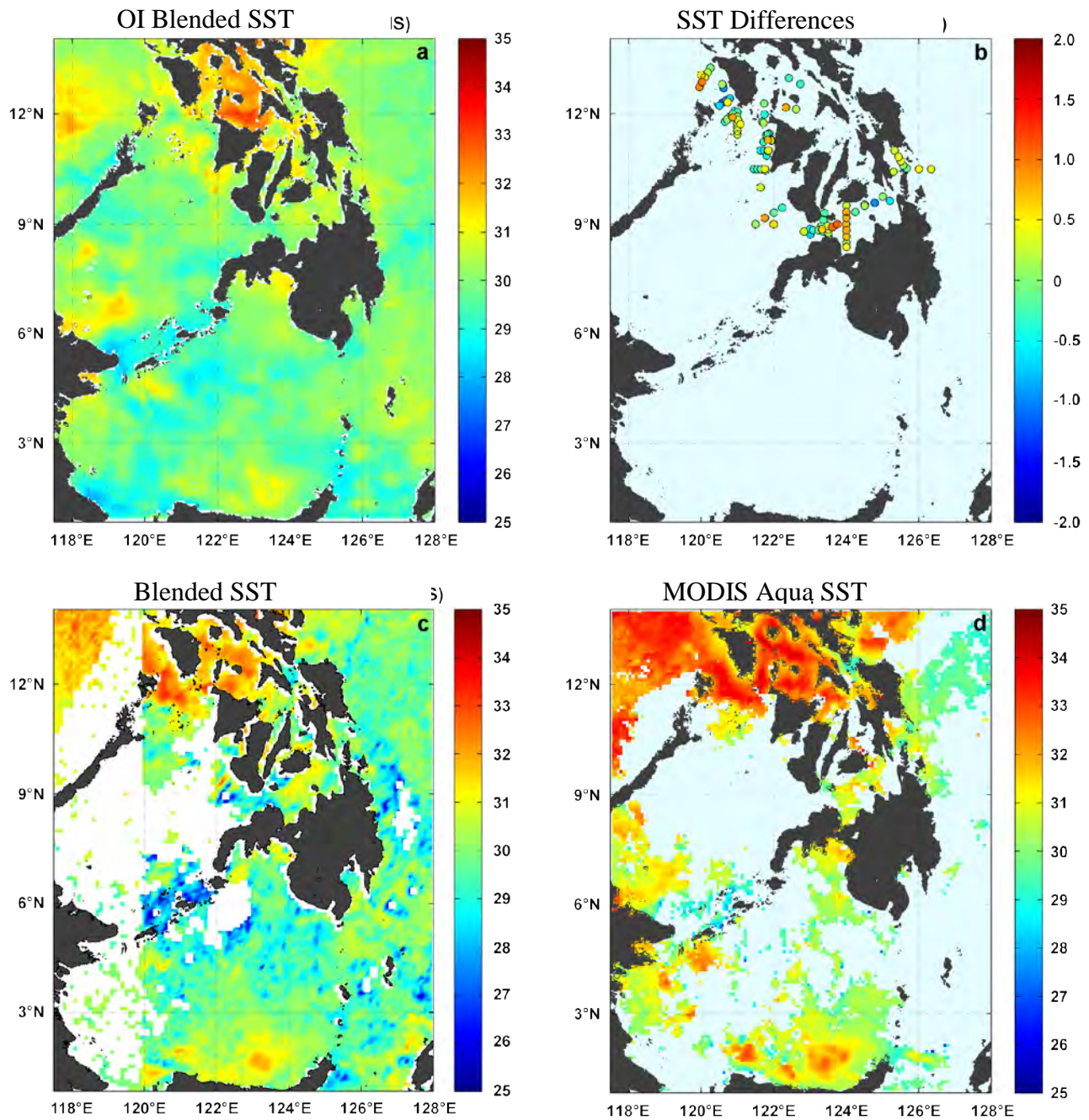
Figure 2: Sample of satellite-derived SST products for 6 Jun 2007: a) gridded OI SST blend from microwave (AMSR-E and TMI) and infrared (MODIS) sensors, b) SST difference ( ^{\circ} C) between surface temperature from Exploratory cruise and OI SST product, c) experimental 5-day SST composite using data from microwave (AMSR-E) and infrared (MODIS, AVHRR, POES, GOES) sensors, and d) SST from MODIS.
