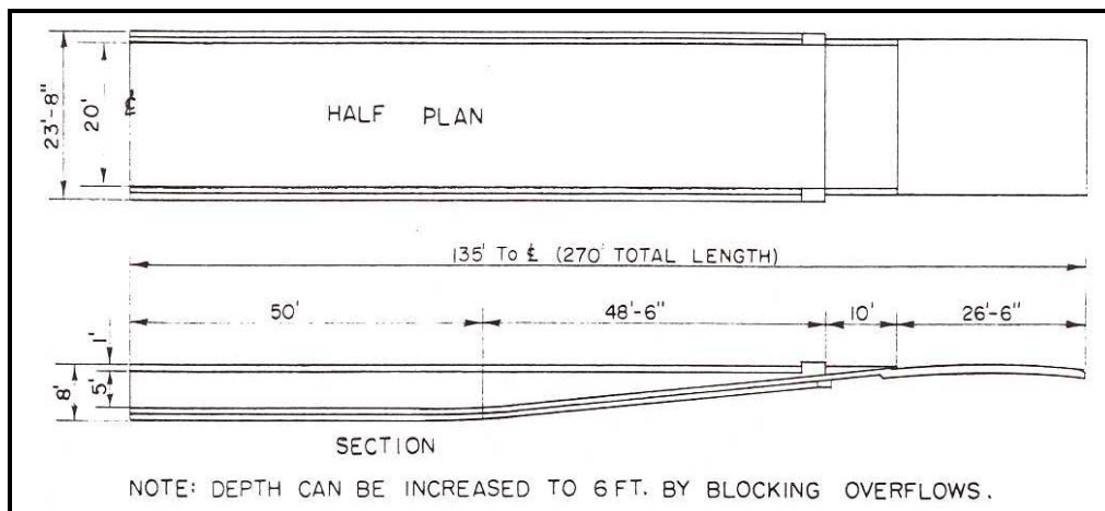
Figure 31. Half plan and section views, Fording Basin.
