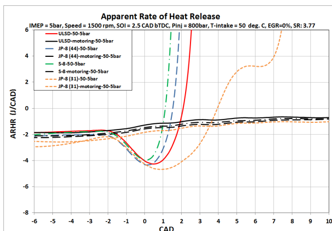
Figure 4: Details of RHR during auto-ignition and early stages of combustion
