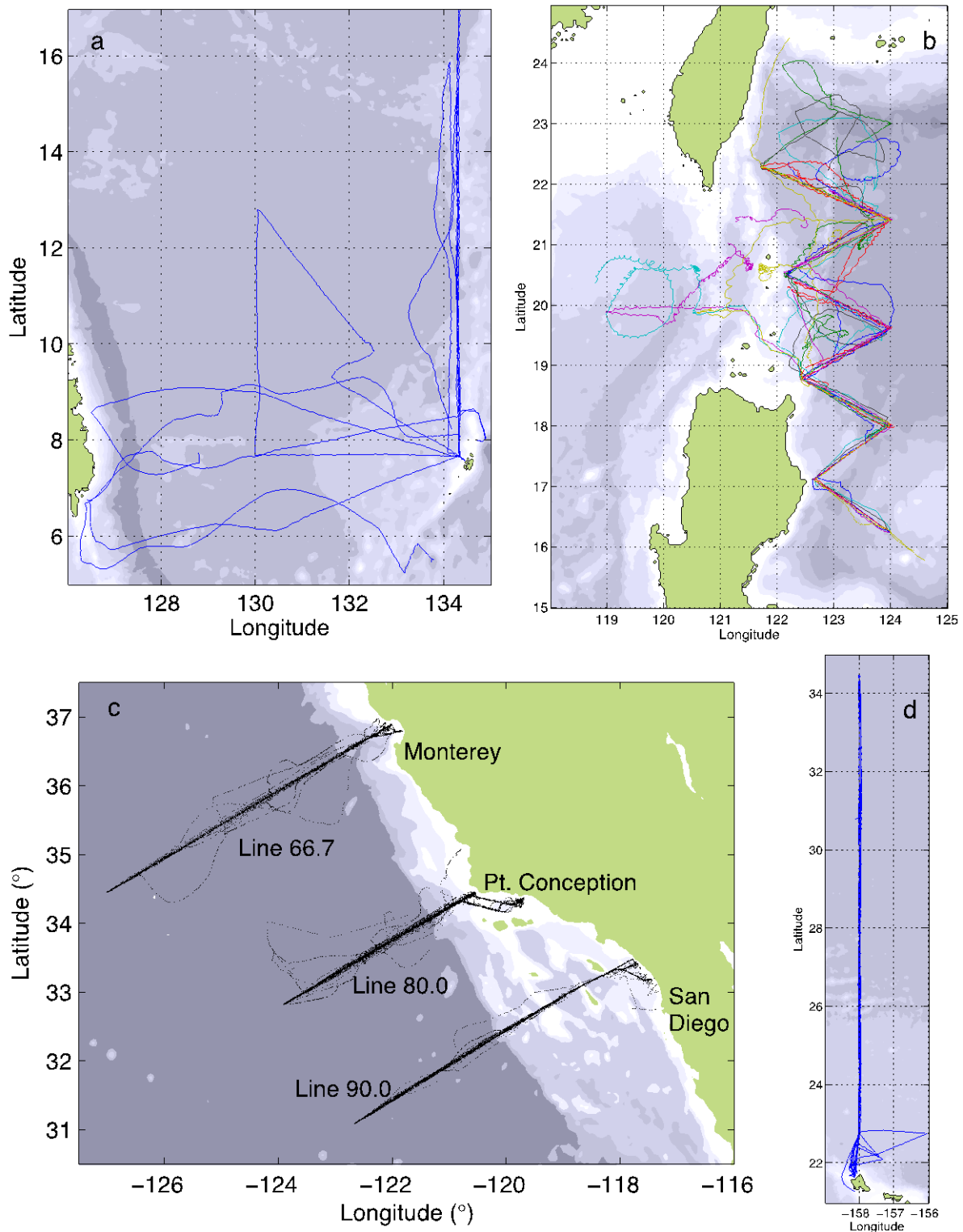
Figure 1. Spray glider trajectories: (a) from Palau into the Mindanao Current and North Equatorial Current, (b) off the Philippines into the Kuroshio near the Luzon Strait and Taiwan, (c) in the California Current System, (d) from Hawaii into the subtropical gyre.
