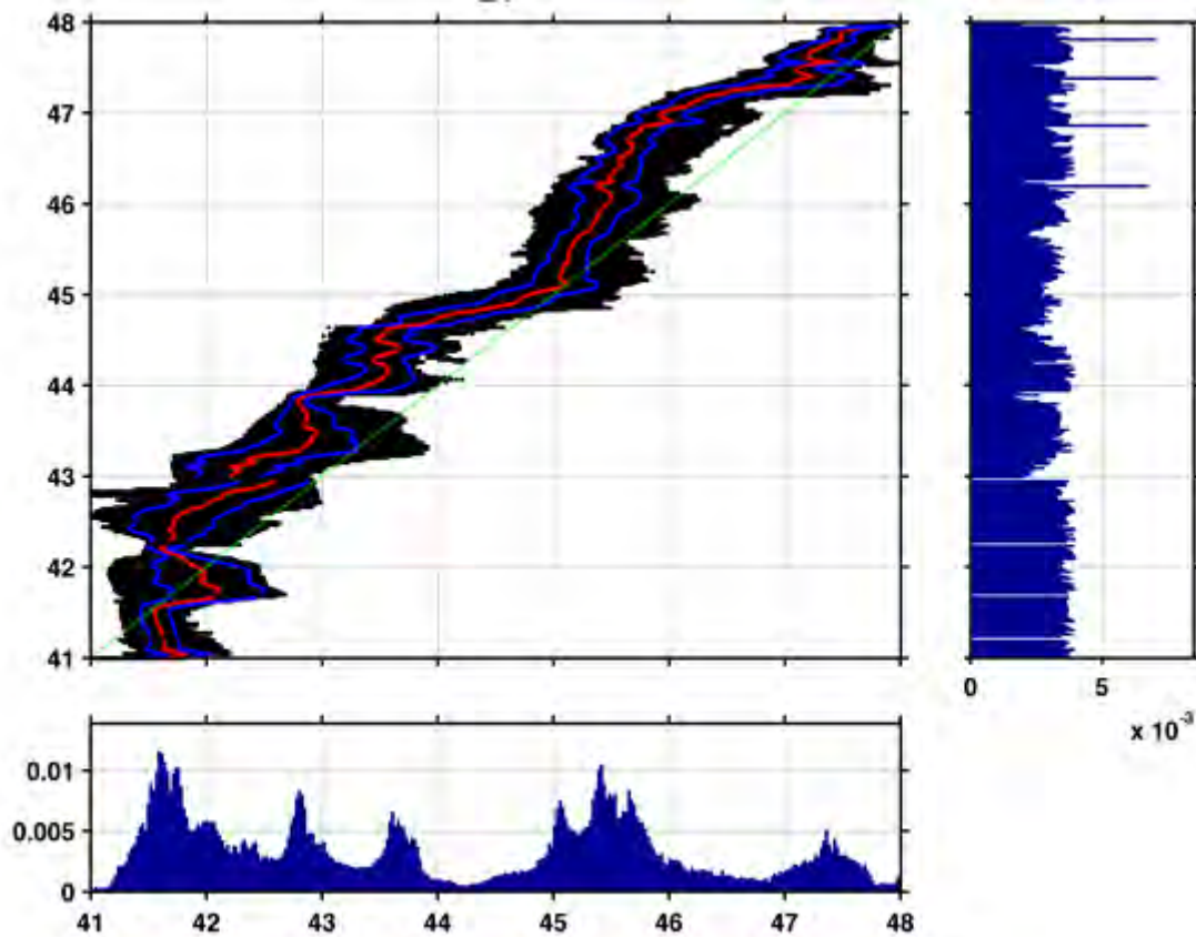
Figure 1. Scatter plot of initial (abscissa) vs. final (ordinate) latitude ( ^{\circ} N) from Lagrangian label advection over one month during summer 2005, for parcels with final positions in the PUC region, where the latter is defined at each latitude as the cross-sectional region between 150 m and 400 m depth within 20 km offshore of the 200-m isobath. The mean (red lines) and mean \pm standard deviation (blue lines) of initial latitude at each final latitude are shown. The distributions show a mean northward displacement of 50-100 km at most latitudes, with mean southward displacements occurring only for final positions south of 42 ^{\circ} N. The histograms along the right and bottom axes show the distributions of label values integrated over the corresponding latitudes; the right-axis histogram thus gives the relative areas of the PUC cross-sectional regions, with some aliasing due to mismatches between the model grid and the histogram bins.
