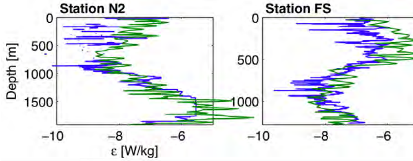
Figure 2: TKE dissipation rate from LADCP/ \chi pod (green) and Thorpe analyses (blue) at two of the most energetic stations observed during the Luzon Strait pilot. These represent the first direct measurements of abyssal turbulence from shipboard CTD/LADCP.
