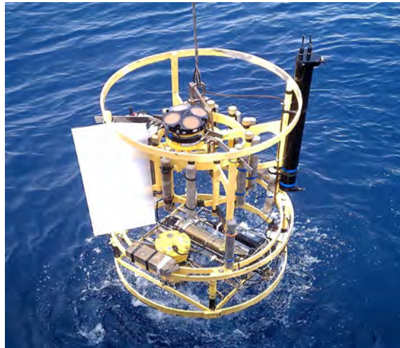
Figure 1: Revelle's CTD as modified during the IWISE pilot to measure full-depth velocity and dissipation rates. 2 ADCPs, a white vane for stabilization, and black \chi pod are each visible.
