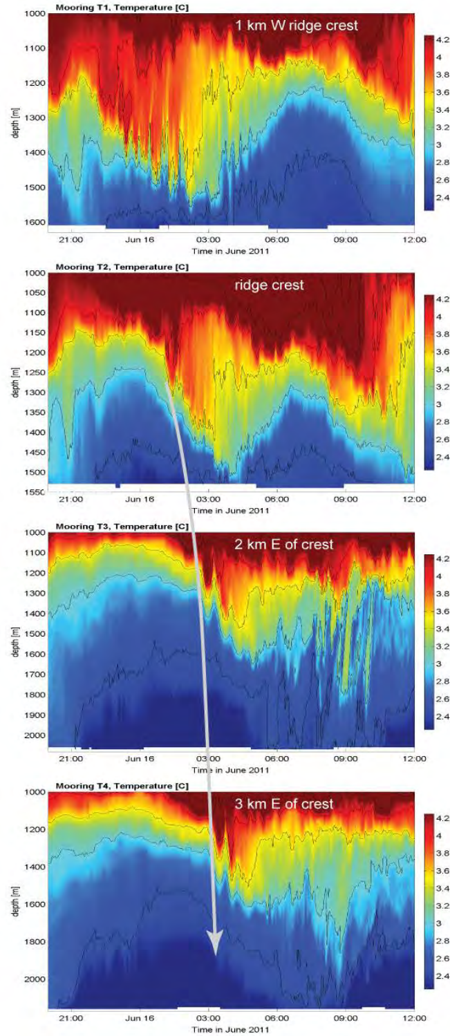
Figure 4: The figure at right shows a 16 h segment of temperature data from the 4 T-chains deployed over the ridge near N2. These moorings were spaced 1 km apart and capture displacements and turbulence in x,z,t space. The depictions at right rival numerical simulations in resolution but capture the represent the true reality and breadth of scales of the real ocean. These figures show the evolution and spatial structure of a 300-m tall wave which grows to 500 m and breaks. Short-wavelength features are coherent across the mooring array and can be tracked (grey arrow). 100-500 m tall turbulent overturns are also visible, particularly at mooring T3 at 0900.
