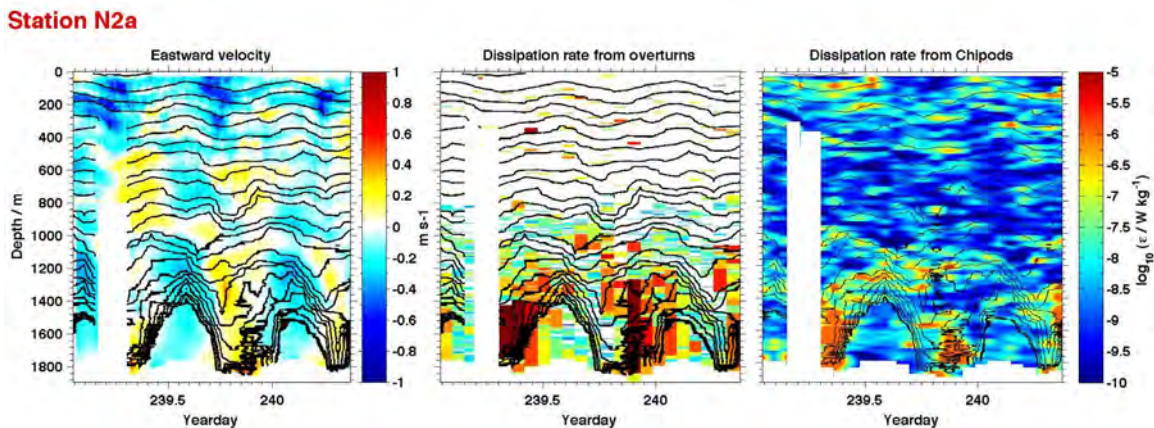
Figure 3 – Timeseries of velocity (left) and TKE dissipation from Thorpe overturns (middle) and from \chi (right) for the first occupation of station N2. This was one of the more energetic stations, with vertical displacements and overturns exceeding 500 m, as illustrated by density contours (black).
