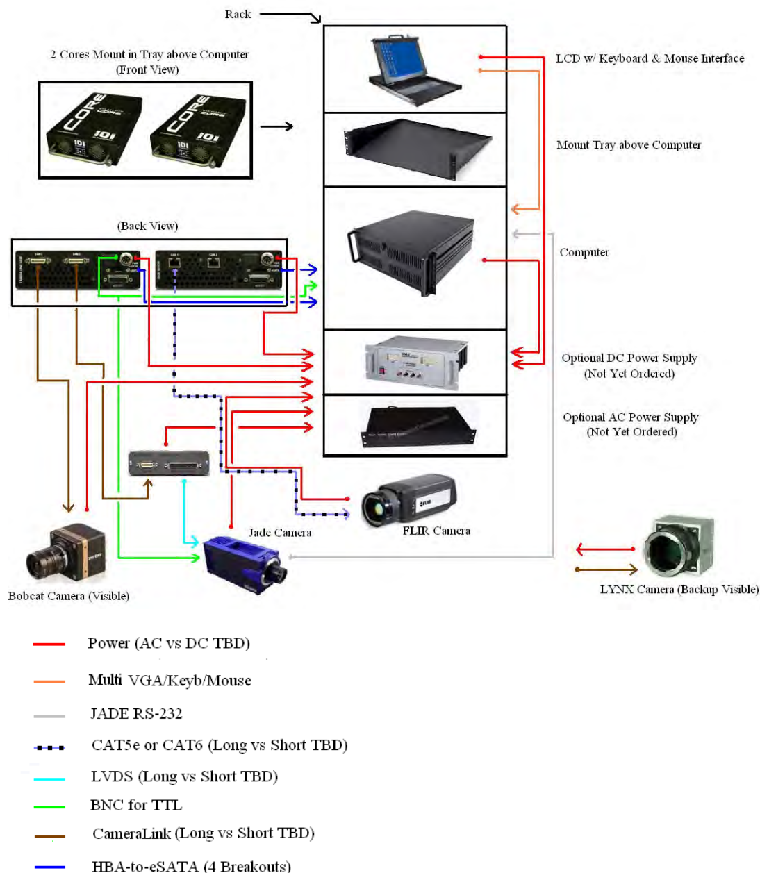
Figure 1. Schematic drawing of the instrument setup and image acquisition system installed on the NOAA P-3 for the LDEO airborne component in DYNAMO program from 3 November 2011 through 15 December 2011.
