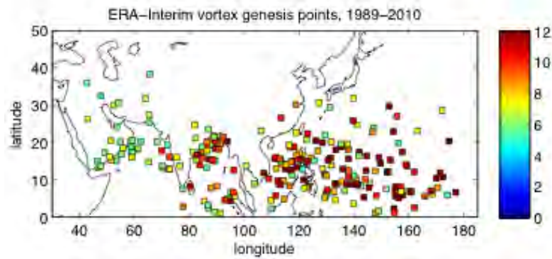
Fig. 2: Genesis sites of vortex tracks for 1989–2010, identified from the ERA-Interim data set using the TRACK algorithm. Color denotes peak relative vorticity ( 10^{-5} \text{ s}^{-1} ) achieved during the life of the vortex.
