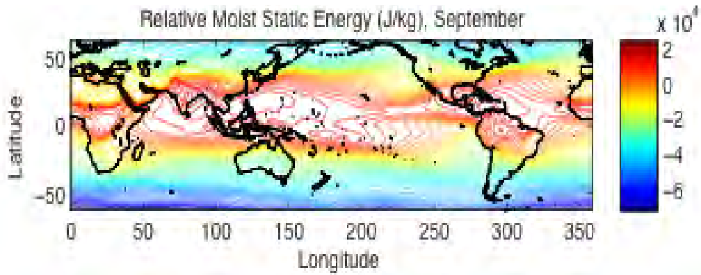
Fig. 3: Climatological mean relative moist static energy for September, from the ERA-40 data set.
