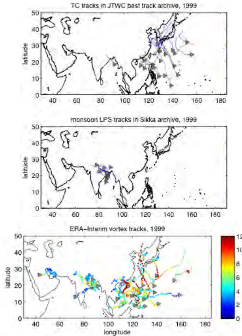
Fig. 1: Cyclonic vortex tracks for 1999. Top: From the JTWC best-track archive. Storms of typhoon intensity are denoted by red lines and weaker storms by blue lines. Triangles denote genesis points. Middle: Tracks from the Sikka (2006) climatology for India. Bottom: Tracks from our identification based on ERA-Interim 850 hPa relative vorticity, using a minimum threshold for vortex strength (not discussed here). Points show 6-hourly vortex centers, with color indicating relative vorticity (in 10^{-5} \text{ s}^{-1} ).
