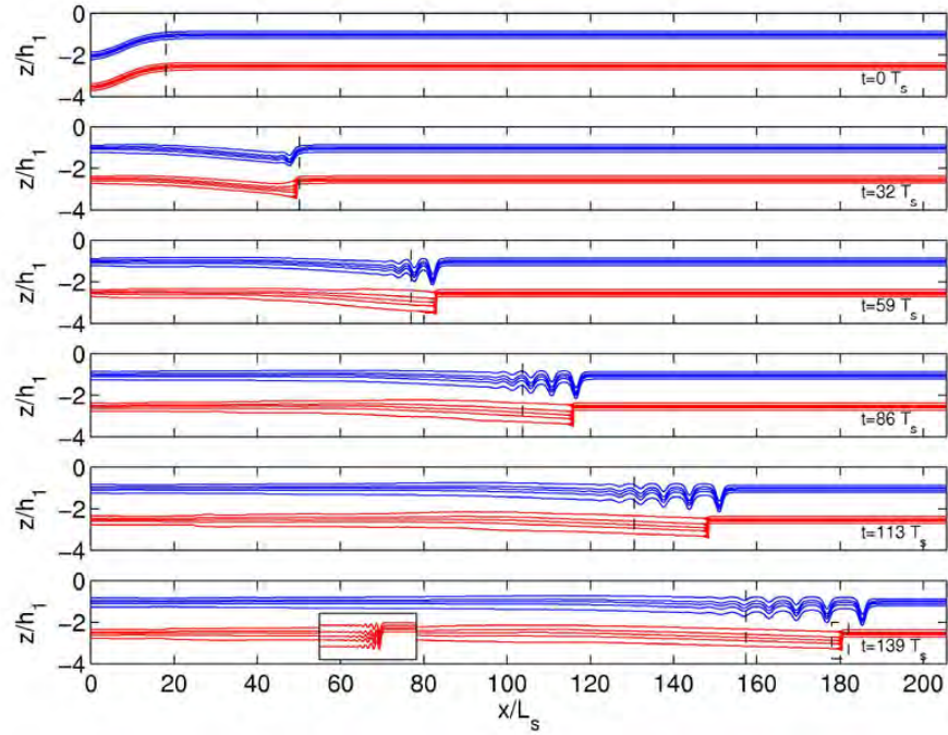
Figure 2: Comparison of the evolution of a solitary-like wave using hydrostatic SUNTANS (red) with nonhydrostatic SUNTANS (blue) with \lambda = \Delta x/h_1 = 0.25 (from Vitousek and Fringer 2011).
