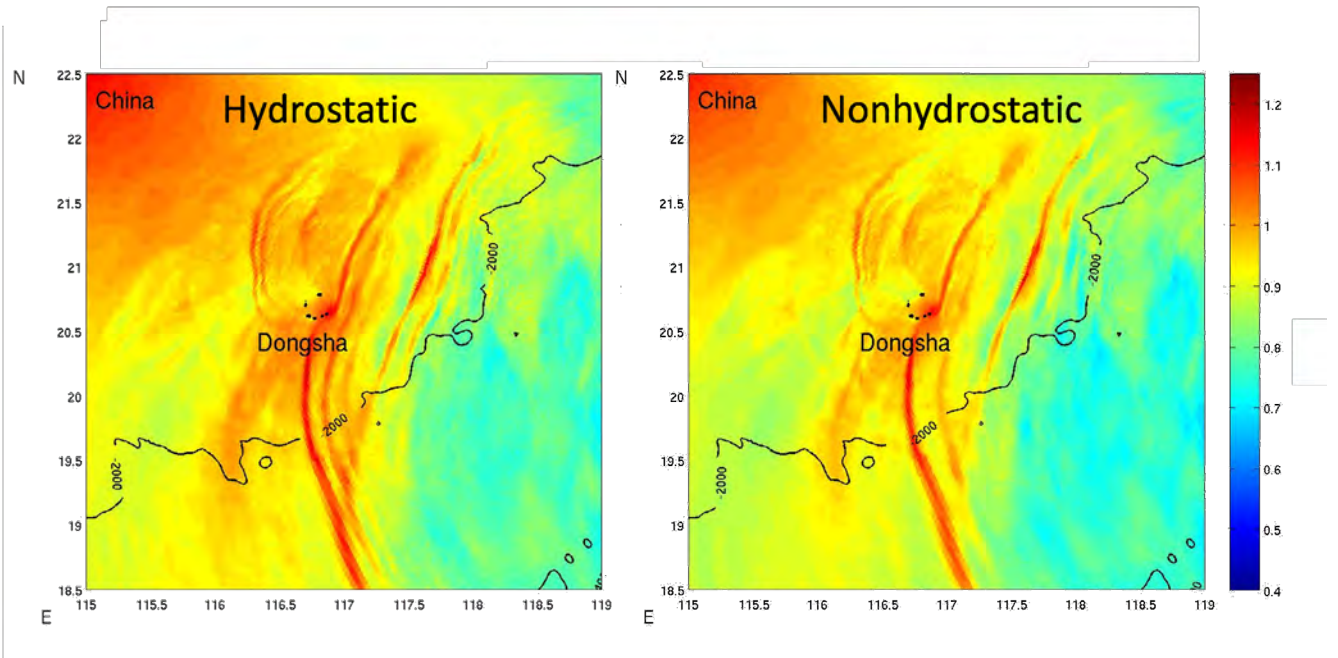
Figure 3: Free-surface displacement (in m above mean sea level) and the associated internal wave signatures at 12:30am on 25 June 2005 around Dongsha Atoll as computed by the hydrostatic (left) and nonhydrostatic (right) versions of SUNTANS (from Zhang et al. 2011).
