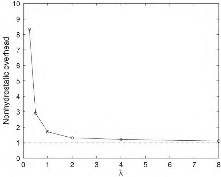
Figure 4: Relative workload associated with computing the nonhydrostatic pressure as a function of the grid lepticity \lambda = \Delta x/h_1 . The overhead is computed as the ratio of the total wallclock time for the nonhydrostatic simulation to that of the hydrostatic simulation to obtain the results shown in Figures 1 and 2 (from Vitousek and Fringer 2011).
