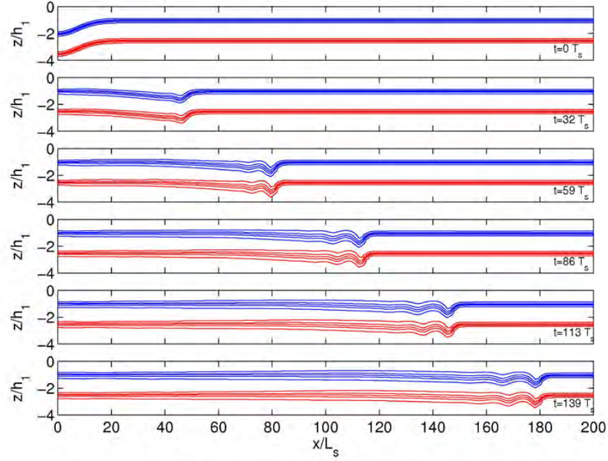
Figure 1: Comparison of the evolution of a solitary-like wave using hydrostatic SUNTANS (red) and nonhydrostatic SUNTANS (blue) with \lambda = \Delta x/h_1 = 8 (from Vitousek and Fringer 2011).
