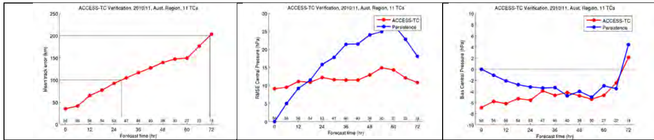
Figure 3: Verification statistics for 11 TCs from the Australian 2010-2011 season. Panels are mean track error (left panel), RMS central pressure error (center) and mean central pressure error (right), every 6 hours to 72 hours. The number of forecasts verified at each time is shown above the x-axis.
