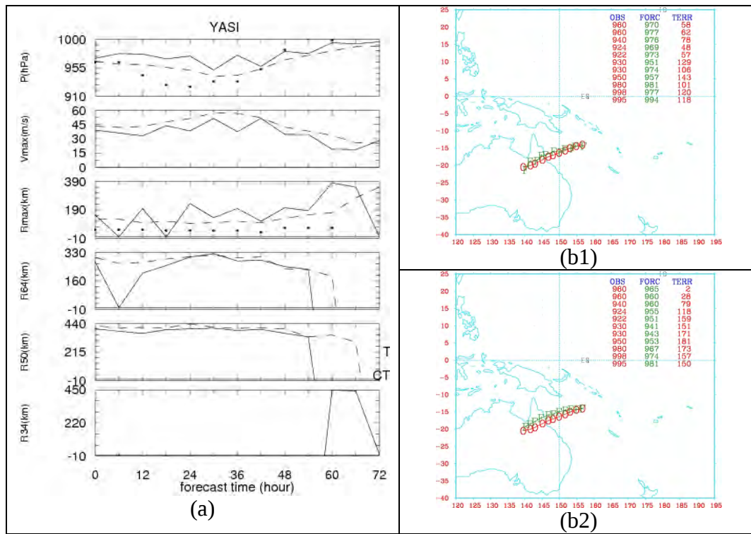
Figure 6. (a) Time series of forecast central pressure, maximum wind, radius of maximum wind, radius of 64, 50 and 34 knot winds, from the original air-sea surface exchange scheme (solid line) and spray route inclusive scheme (dashed line). In (a), the solid line refers to the original scheme and the dashed line is to the spray route scheme. The dot symbols in the top frame are operational estimates of central pressure. Panel (b1) plots the observed and forecast tracks and tabulates the observed and forecast central pressures (hPa) and track errors (km) at 6-hour intervals from the standard scheme. Panel (b2) is similar, except for the new scheme.
