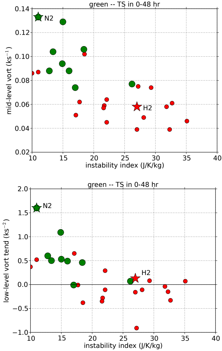
Figure 4: Mid-level vorticity (upper panel) and low-level vorticity tendency (lower panel) as a function of instability index for a combination of TCS-08 and PREDICT case studies of potential tropical cyclones.
