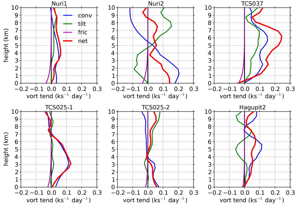
Figure 2: Mean profiles of total vorticity tendency (red) and its individual components (blue: vorticity convergence; green: tilting; magenta: friction) for all missions except TCS030.
