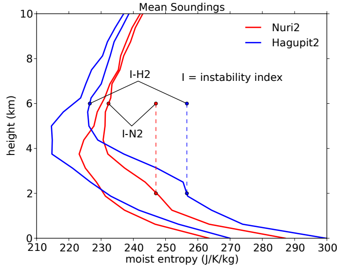
Figure 3: Soundings for developing (Nuri2) and stagnating (Hagupit2) disturbances. The instability index for the developing case is much smaller.
