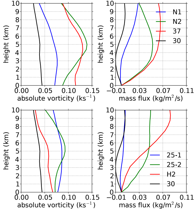
Figure 1: Vertical profiles of absolute vorticity (left panel) and vertical mass flux (right panel) area-averaged over selected analysis regions. The upper panels show Nuri1, Nuri2, TCS037, and TCS030, while the lower panels show TCS025-1, TCS025-2, and Hagupit2. (TCS030 is included for comparison purposes.)
