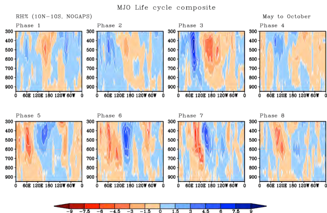
Figure 9 Same as Fig. 8 except for relative humidity from NCEP2.
