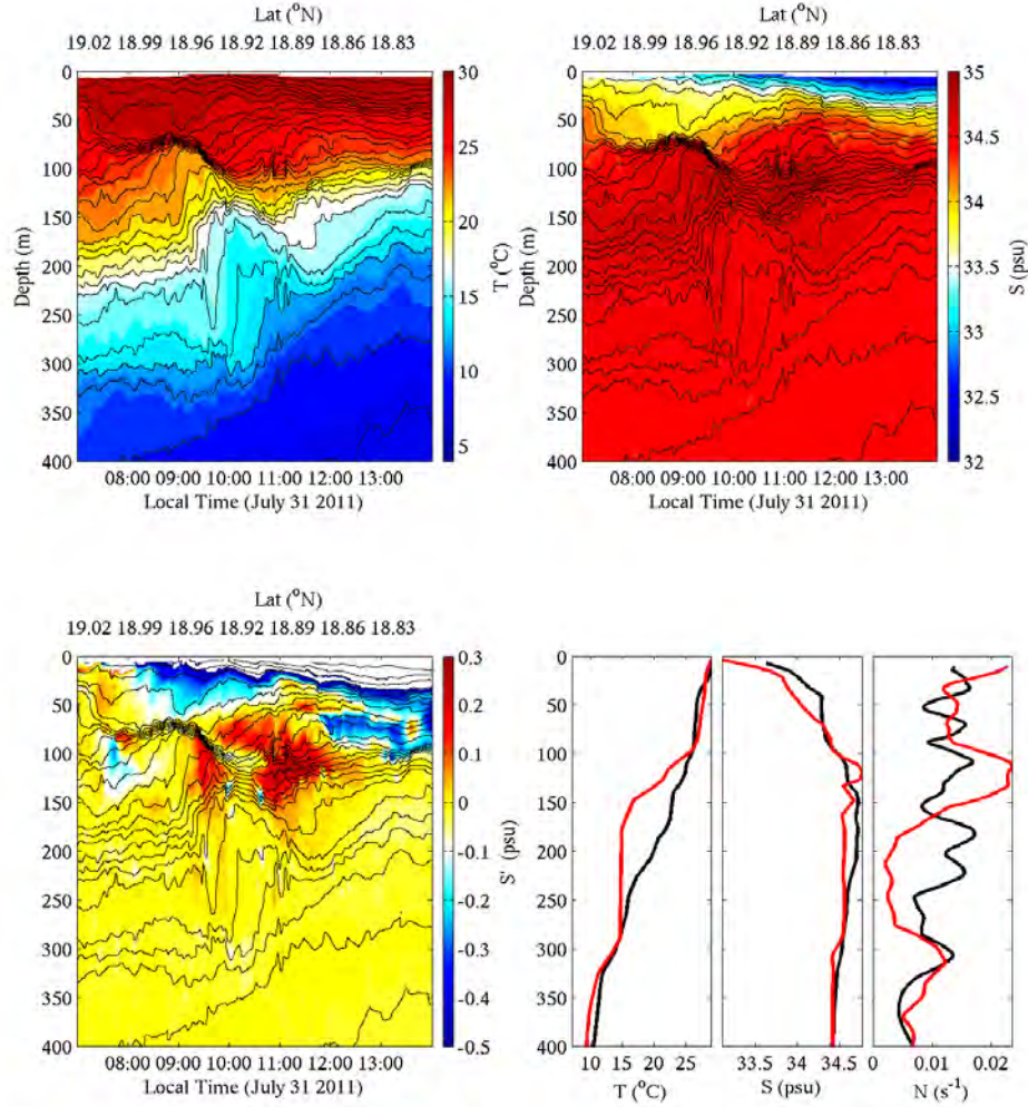
Figure 5: Example of hydraulic jump feature west of the channel between Dalupiri and Fuga islands. The color shadings in the top two panels show the salinity and temperature, and the contour lines represent isopycnals. In the bottom left panel, the color shading shows the salinity anomaly referenced to the T – S relation at 07:00 on 31 July 2011, and the contour lines represent isopycnals. The bottom right group of three panels shows vertical profiles of temperature, salinity and buoyancy frequency at 07:00 (black curves) and in the middle of hydraulic jump (red curves).
