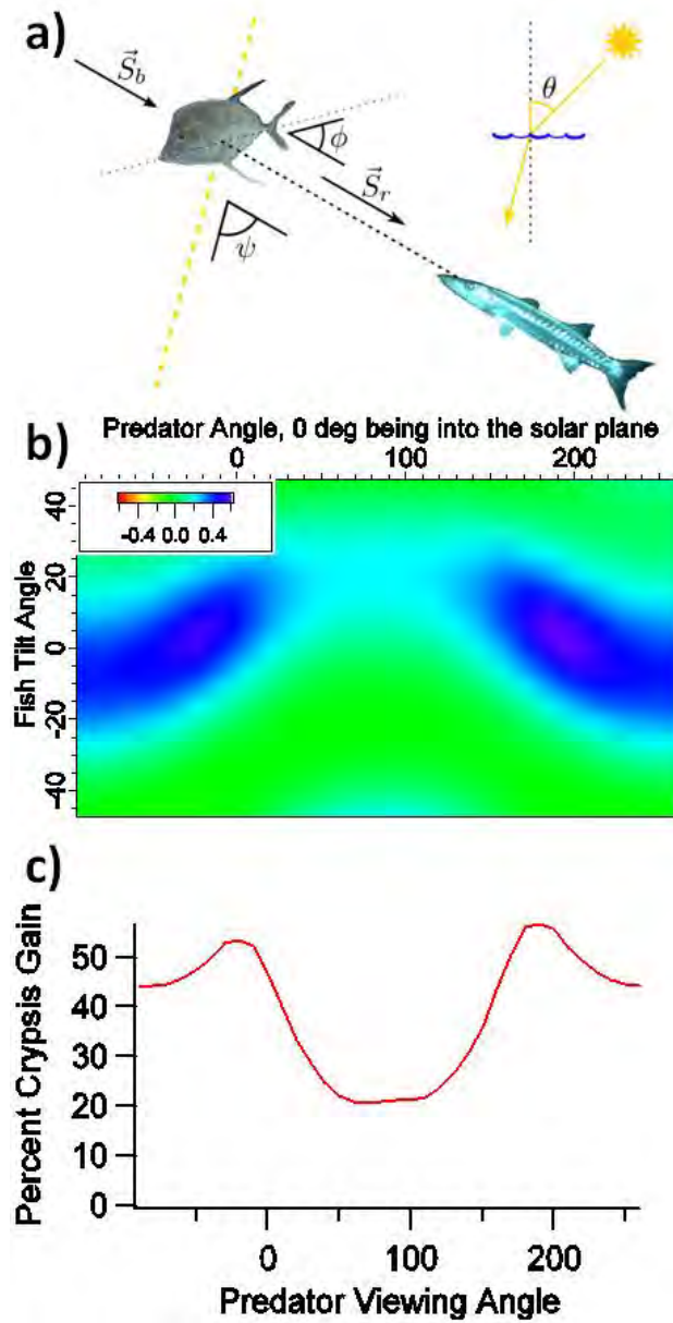
Figure 7. We model the polarization reflections of the fish using Mueller matrices measured from the Lookdown (See Fig 6). We evaluate polarocrypsis as the contrast ratio or the RMS difference between the target reflected Stokes vector ( \vec{S}_r ) and the background Stokes vector ( \vec{S}_b ) at solar elevation of \theta = 60^\circ . (a) Three angles parameterize the contrast ratio calculation: \theta , the angle between the sun and the zenith which defines the solar plane (indicated by the dotted orange line in the figure); \psi , the predator's observation angle with respect to the solar plane; and \phi , the angle between the surface of the prey and the predator's observation angle. (b, c) We calculate the percent crypsis gain ( PG = 100 \times (G_{\text{Lookdown}} - G_{\text{verticalmirror}}) / G_{\text{verticalmirror}} ) between an idealized mirror and the lookdown fish Mueller matrix, where G = \|\vec{S}_b - \vec{S}_r\|^{-1} . We assume that the Mueller matrix rotates roughly invariantly with the angle \phi , as our measurements indicate this to an approximation. (b) Percent crypsis gain (PG) across a range of fish tilt angles ( -45^\circ to 45^\circ ) for all possible predator viewing angles ( \psi = 0^\circ to 360^\circ ). (c) the PG for the optimal fish tilt from (b).
