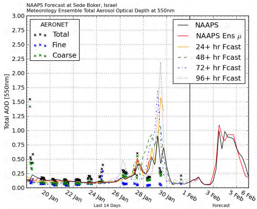
Figure 3. Example verification plot showing NAAPS, eNAAPS forecast data against AERONET sun photometer data for the January 29 th 2011 dust event.
