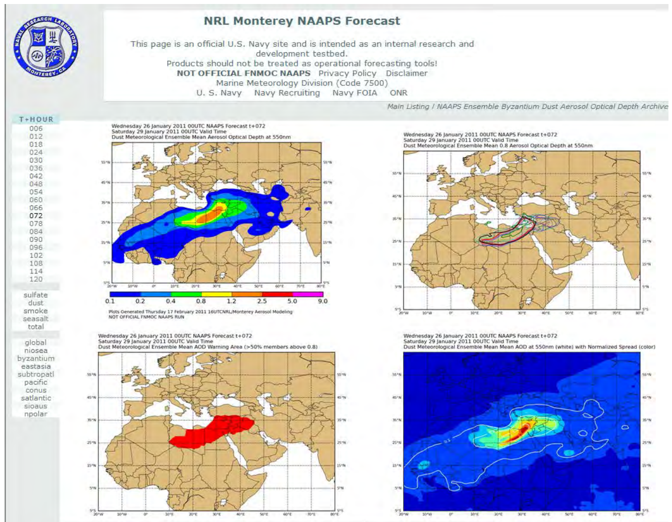
Figure 1. Example output for the quasi-operational ensemble NAAPS (eNAAPS) from the NRL aerosol website. Shown in the 72 hour forecast initiated on January 26 st for the Africa/Europe domain. Given are (upper left) ensemble mean, (upper right) spaghetti plot for aerosol optical depth >0.8, (lower left) dust warning area where 50% or more members predict dust optical depths >0.8, and (lower right) mean and standard deviation of the ensemble AODs.
