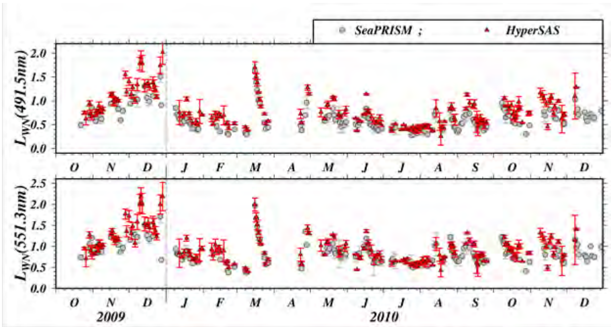
Fig. 1. Time series of daily average of the exact normalized water-leaving radiance (in \text{mW cm}^{-2} \text{sr}^{-1} \text{nm}^{-1} ) retrieved with HyperSAS (red triangles) and SeaPRISM (grey circles) for two SeaPRISM bands centered on 551 and 491 nm. The vertical bars correspond to the daily standard deviations.
