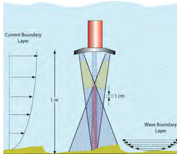
Figure 3. Schematic diagram of the pulse-coherent Doppler sonar system developed at WHOI by Austin, Jaffre, Terray & Trakovski. The red shaded area represents the region that would be profiled at turbulence resolving rates ( \sim 10 Hz) and the extended yellow region would be profiled at a slower rate ( \sim 2 Hz). An additional pair of angled transducers is located in the plane perpendicular to the pair shown.
