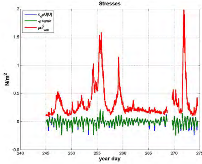
Figure 1. Stresses estimated from the 2007 measurements at the Martha's Vineyard Coastal Observatory. The directly measured hour-averaged Reynolds shear stress -\rho \langle uw \rangle agrees well with the drag-law estimate c_d \rho |U| U inferred from the measured burst-averaged velocity U by means of an empirically determined drag coefficient c_d . The standard deviation \rho u_{*wm}^2 of the oscillatory bottom shear stress produced by surface waves is inferred from a wave-current interaction model and is much larger than the hour-averaged stress -\rho \langle uw \rangle , which is associated with wind-driven and tidal currents. The wave-induced stress is primarily responsible for suspending particles and controlling the size of water-borne flocs.
