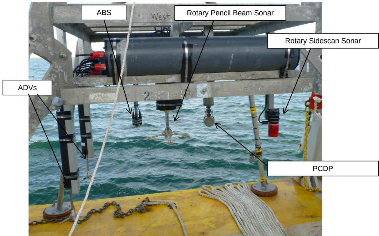
Figure 4. Photograph of instrumentation just before deployment at MVCO in September 2011, showing Pulse Coherent Doppler Profiler (PCDP), Imagenex rotary sidescan sonar, Imagenex 2-axis rotary pencil beam sonar, Aquatec ABS and Nortek Vector ADVs.
