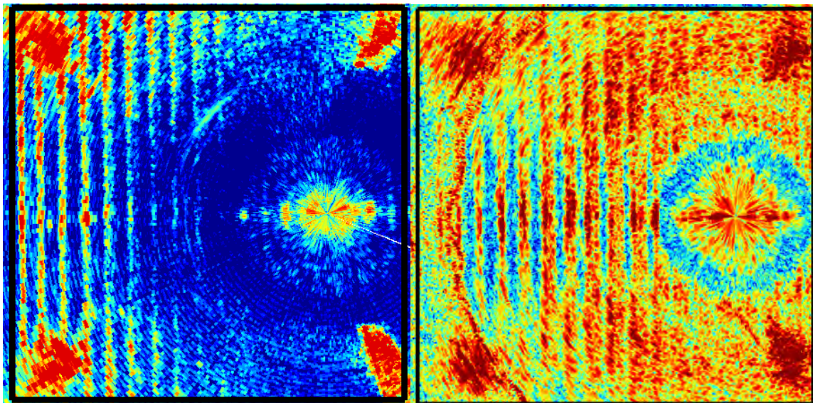
Figure 5. Data from two prototype 881L tilted head rotary fanbeam sonars. The data in the right panel uses a wider beamwidth transducer to increase the ability to image under the sonar. The size of the imaged box is 2.5 m on a side.
