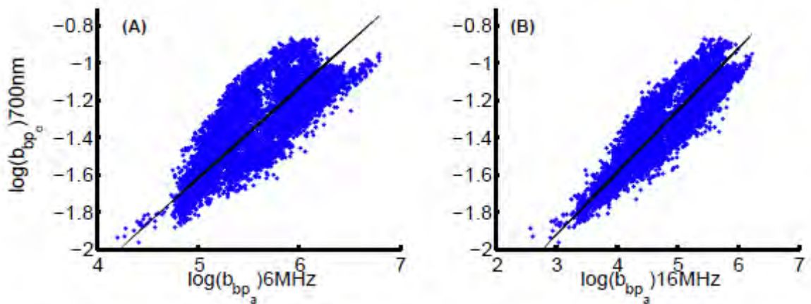
Figure 2. Comparison of acoustical and optical backscattering in the bottom boundary layer for two different acoustical frequencies.
