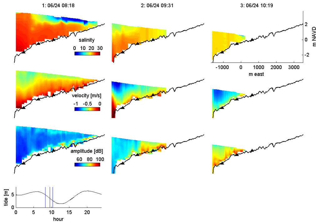
Figure 4. Three across-flats surveys of salinity (top), velocity (middle), and acoustic backscatter (bottom) during a spring ebb tide. Tidal elevation is in the lower left with survey times shown; stations 1, 2, and 5 are marked with triangles on the transects. The sloping water surface reflects the change in tidal elevation during each transect. In transect 1, strong stratification, strong velocity shear, and low acoustic backscatter extended across most of the flats. In transect 2, stratification remained strong on the lower flats (west of station 2), but on the upper flats the water column was vertically mixed, had less shear, and had higher backscatter. By transect 3, the well-mixed, high-backscatter region extended to the edge of the flats. This breakdown of stratification and increase in backscatter was also recorded at the quadpods, similar to that in Fig. 6.
