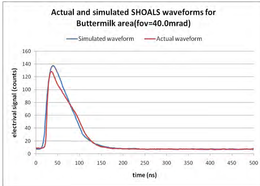
Figure 4. Comparison plot of simulated waveform and actual SHOALS for Buttermilk Bay, MA.
