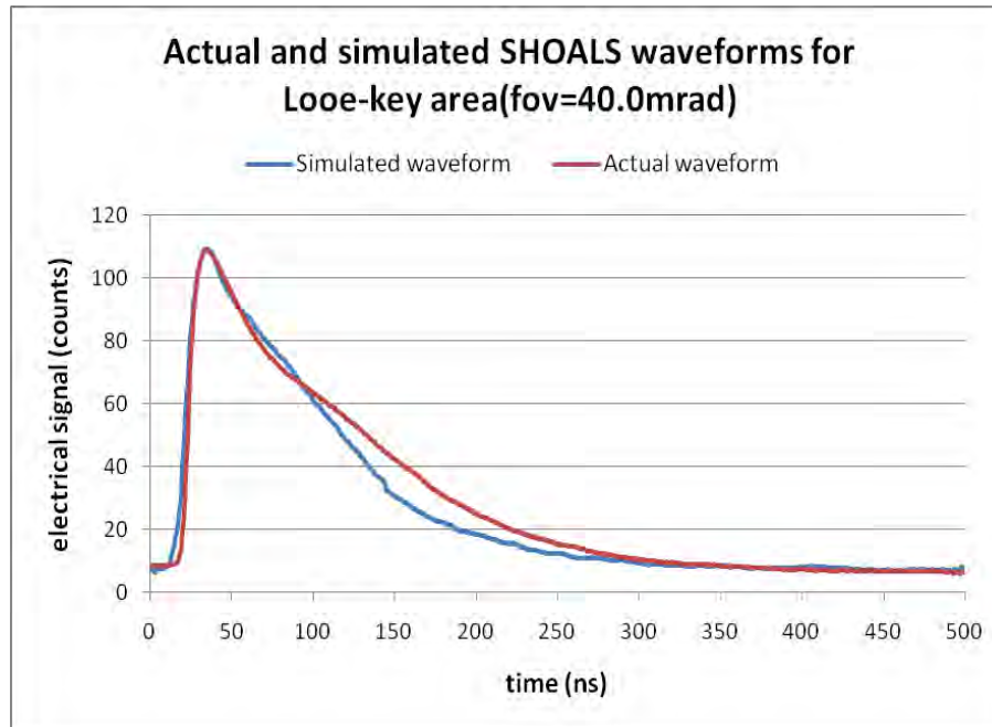
Figure 3. Comparison plot of simulated waveform and actual SHOALS for Looe Key, FL.
