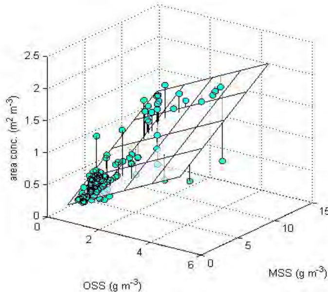
Figure 2. Area concentration in suspension versus organic suspended sediment concentration (OSS) and mineral suspended sediment concentration (MSS). Data are from Dave Bowers at the University of Bangor in Wales. They were collected in a range of coastal environments. The plane shows the best fit linear regression of area concentration on OSS and MSS. If particle composition is uncorrelated with the packing geometry of flocs, then the ratio of the regression coefficient for OSS to the regression coefficient for MSS should equal the ratio of densities between mineral matter and organic matter. Assuming a mineral density of 2650 \text{ kg m}^{-3} and a bulk organic density of 1370 \text{ kg m}^{-3} , the predicted ratio of coefficients is 1.93. The observed ratio is 2.12 and is not significantly different from 1.93. This result suggests that compositional variability accounts only for a 2x range of variability in the c_p :SPM ratio
