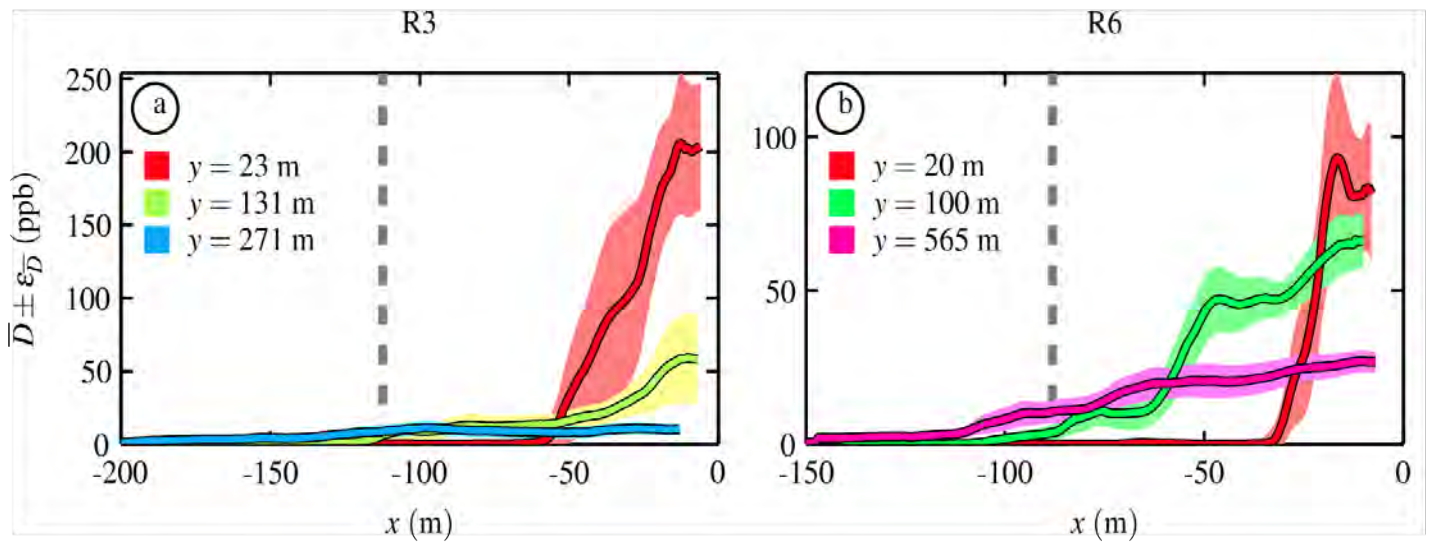
Figure 2: Mean dye profile curves D(x; yj) with lighter regions indicating range of D(x; yj) included in the average, for dye releases (a) R3 and (b) R6 at three alongshore distances y from the dye source (see legend). The dashed gray line indicates the seaward edge of the surfzone. Vertical scales differ.
