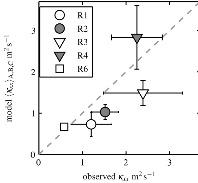
Figure 6 Mean modeled \langle \kappa_{xx} \rangle_{A,B,C} versus observed \kappa_{xx}^{(\text{obs})} , with a dashed line indicating perfect agreement. The \kappa_{xx}^{(\text{obs})} error bars are estimated from the \sigma_{\text{surf}}^{2(\text{obs})} versus t_p fit slope error [Clark et al. , 2010], and model \langle \kappa_{xx} \rangle_{A,B,C} error bars are the combination of fit slope errors and the variation in \kappa_{xx}^{(A,B,C)} magnitudes. The skill is 0.40.
