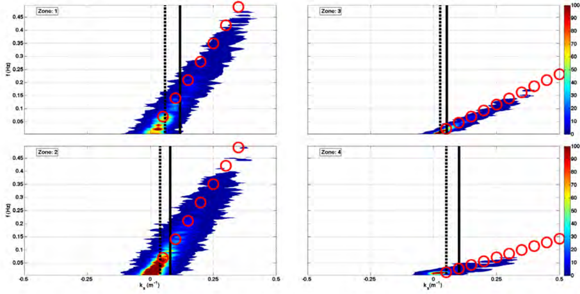
Figure 3. Frequency-wavenumber spectra for the streamwise ADB velocities measured within the four different zones. The red circles represent the mean velocity. Vertical lines represent two (solid) or four times (dashed) the maximum array length. Normalized velocity colorscales plotted to the right.
