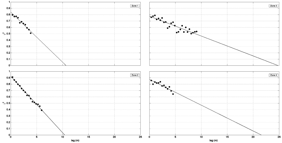
Figure 4. The mean coherency as function of lag. Solid lines represent least-square linear fit. Y-intercepts represent coherent lengths.
