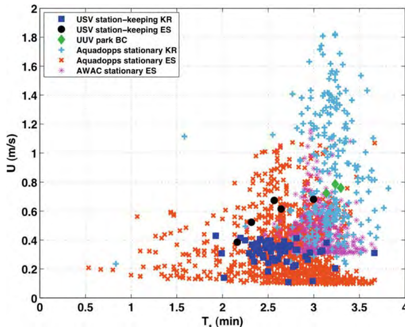
Figure 5. Depth-averaged flow velocity magnitude versus depth-averaged averaging window, T^* , measured by ADCPs mounted on various stationary platforms in differing environments
