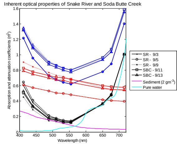
Figure 10. (a) Diffuse attenuation coefficient K_d spectra computed from vertical profiles of downwelling spectral irradiance measured along the Snake River and Soda Butte Creek. A K_d spectrum from the much more turbid Platte River is also shown for comparison. (b) Inherent optical properties measured with an ac-9, along with absorption coefficient values for pure water and suspended sediment. The absorption, scattering, and attenuation coefficients a , b , and c are represented by the black, red, and blue lines, respectively, with different symbols for each site/date.
