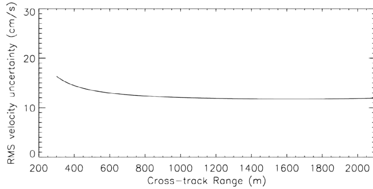
Figure C1: Predicted rms velocity uncertainty for the microASAR operating at an altitude of 600 m, a nominal incidence angle of 60^\circ , and a squint angle of 30^\circ . The cross-track swath extends from 300 to 2100 m. The normalized radar cross section is computed from the CMOD5n model function (CMOD5 for neutral winds) for a wind speed of 2 \text{ m s}^{-1} with the radar looking nominally upwind.
