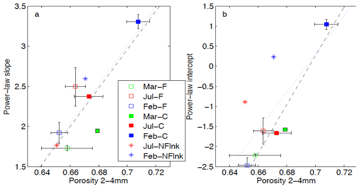
Figure 9. Correlation between average porosity 2-4 mm below the sediment surface ( P_{24} ) and the a) slopes (PLS) and b) intercepts (PLI) of power-law fits to average cumulative mass eroded vs. bed shear stress (Table 4). Both correlations are significant ( p < 0.05 ). The horizontal and vertical bars show standard error for each parameter, with the exception of C-Channel in March 2009 (Mar-C) and the northern channel flank in July 2009 and February 2010 (Jul-NFlnk and Feb-NFlnk) for which values for only one sampling site are available. The regressions equations (dashed lines) for the flat and channels averages are PLS = 23.9 \cdot P_{24} - 13.8 ( r^2 = 0.69 ) and PLI = 60.7 \cdot P_{24} - 42.4 ( r^2 = 0.92 ). The dotted regression lines, which include the channel flank sites as well, are also significant, with r^2 = 0.69 for PLS and r^2 = 0.52 for PLI.
